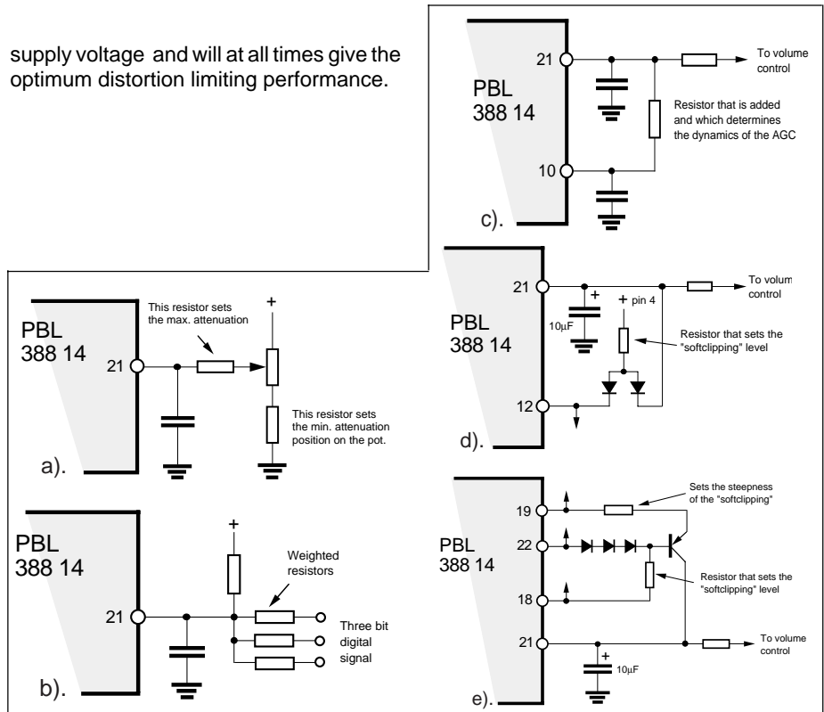
Figure 17. DC - volume control options.
