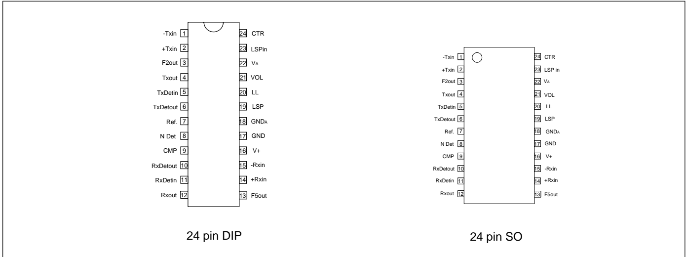
Figure 4. Pin configuration.
