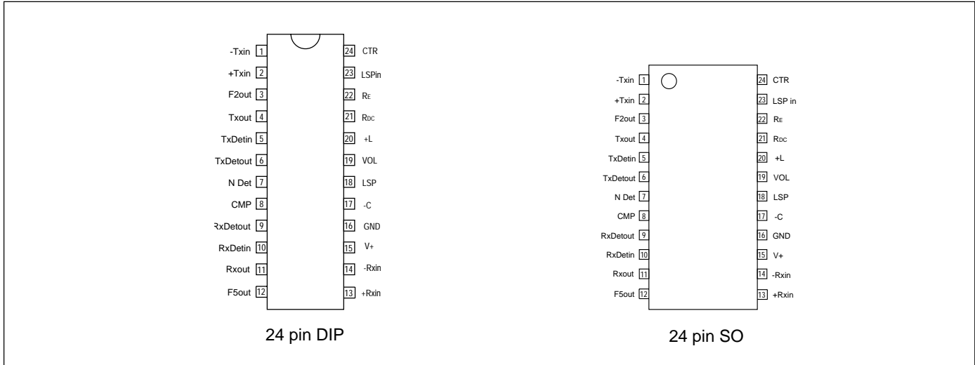
Figure 6. Pin configuration.
