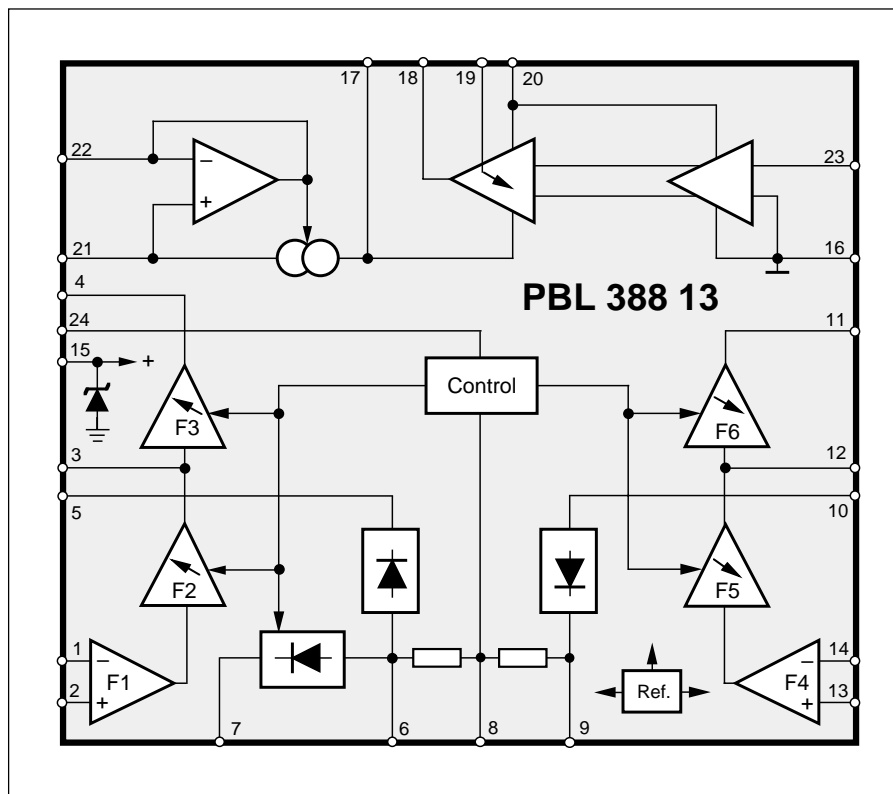
Figure 1. Block diagram.
