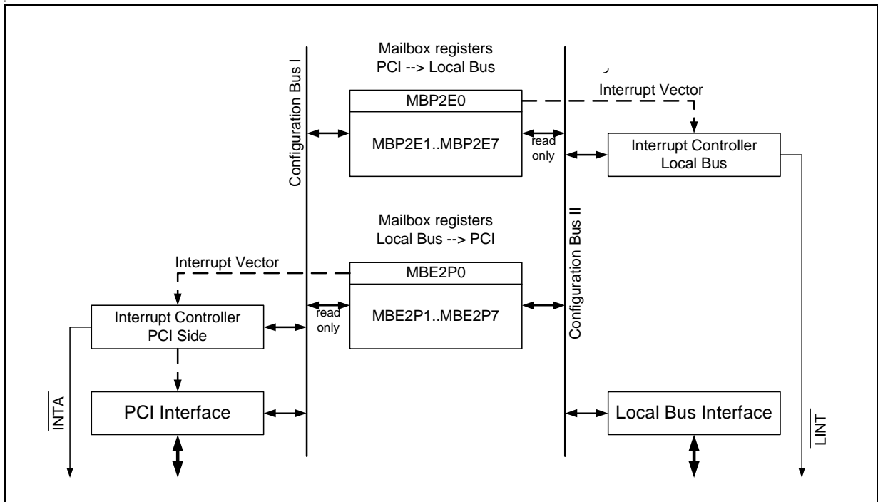
Figure 4-16 Mailbox Structure
