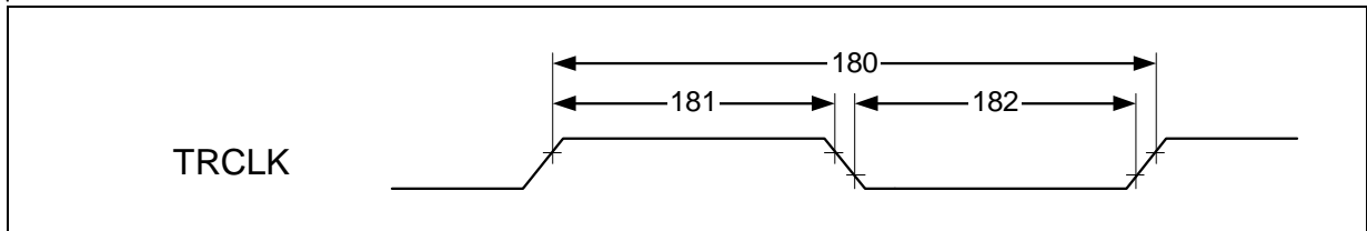
Figure 9-33 T1/E1 Test Receive Clock Timing
