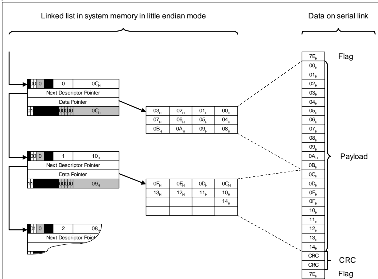
Figure 4-6 Descriptor Structure
