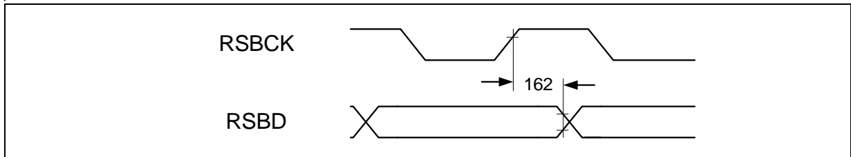
Figure 9-28 DS3 Receive Stuff Bit Timing
