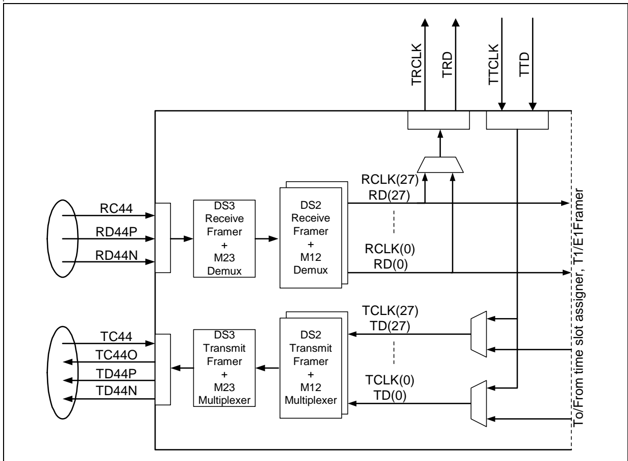
Figure 4-4 Test Breakout
