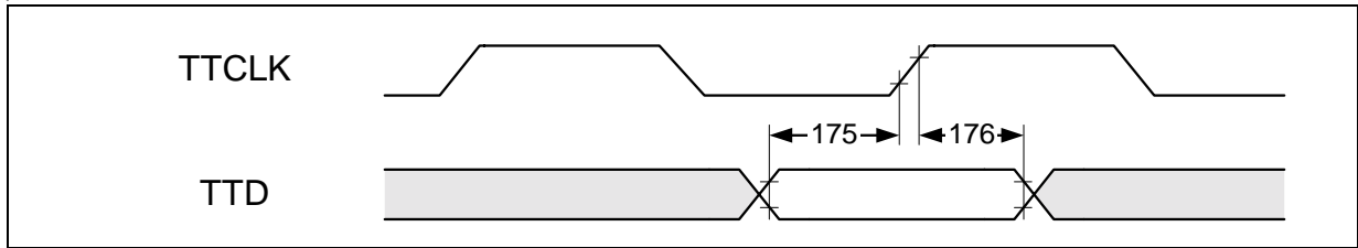
Figure 9-32 T1/E1 Test Transmit Data Timing
