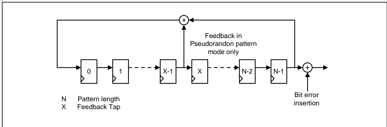
Figure 4-15 Pattern Generator
