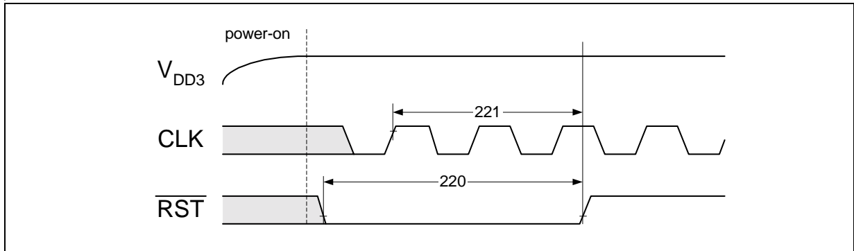
Figure 9-36 Reset Timing
