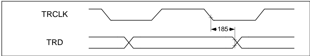
Figure 9-34 T1/E1 Test Receive Data Timing
