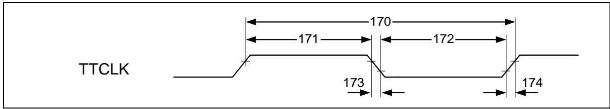
Figure 9-31 T1/E1 Test Transmit Clock Timing
