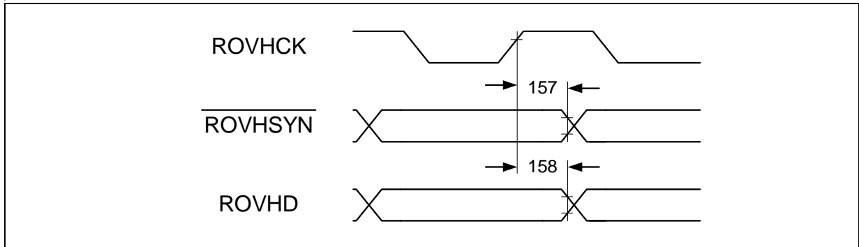
Figure 9-26 DS3 Receive Overhead Timing
