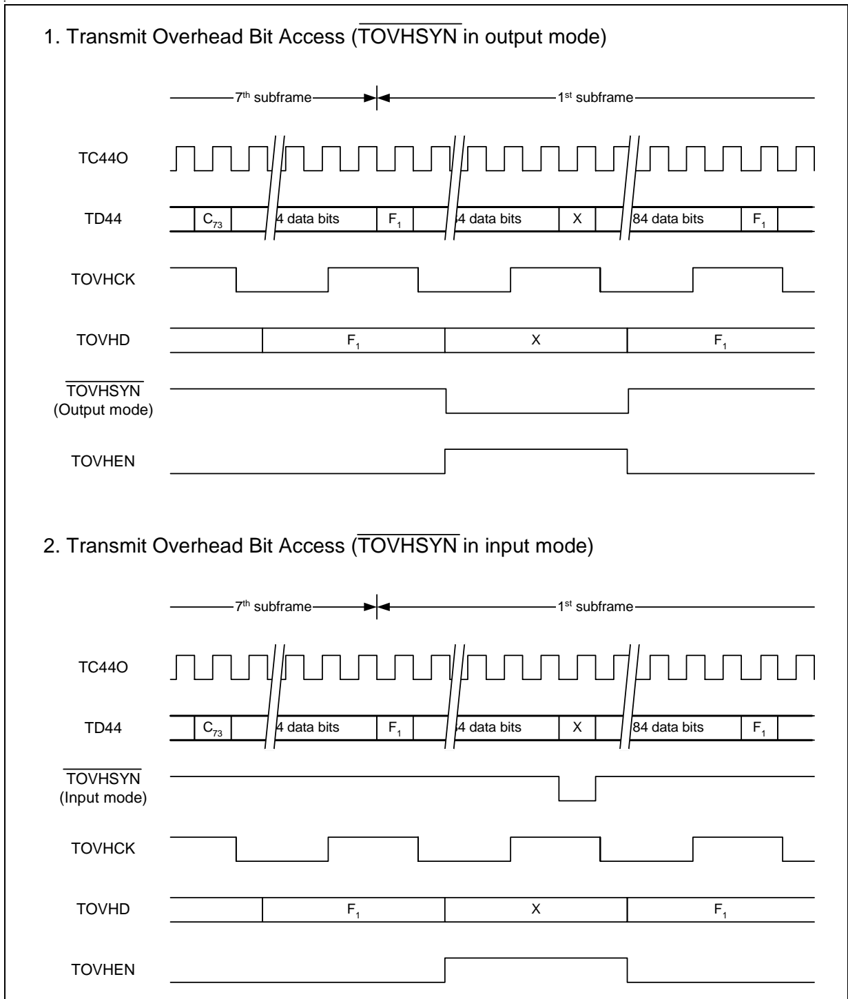
Figure 5-10 Transmit Overhead Access
