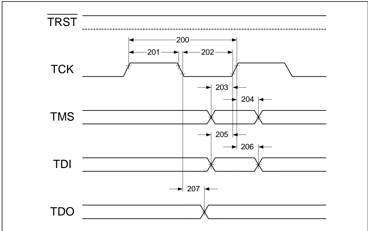
Figure 9-35 JTAG Interface Timing
