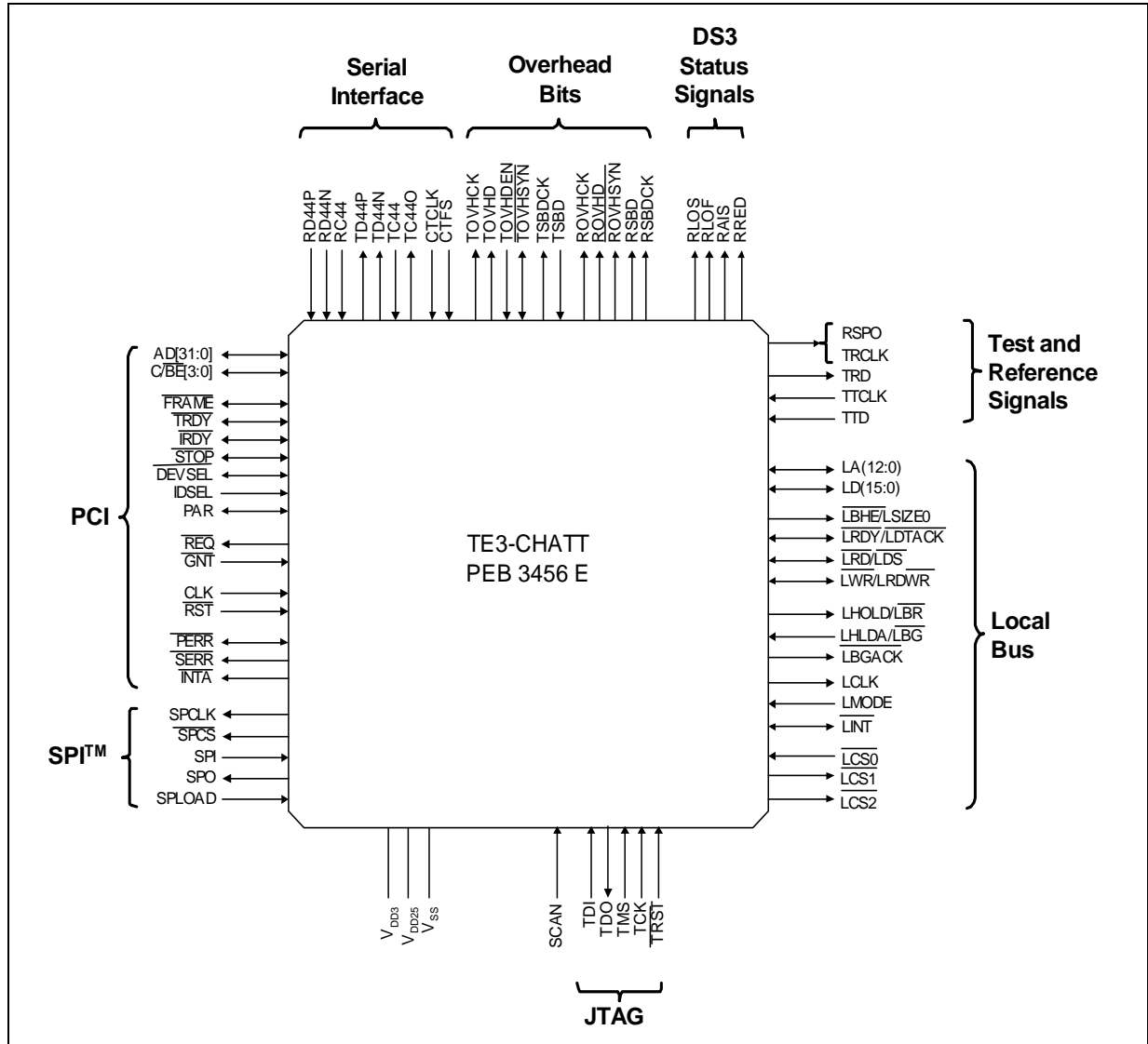
Figure 1-1 TE3-CHATT Logic Symbol
