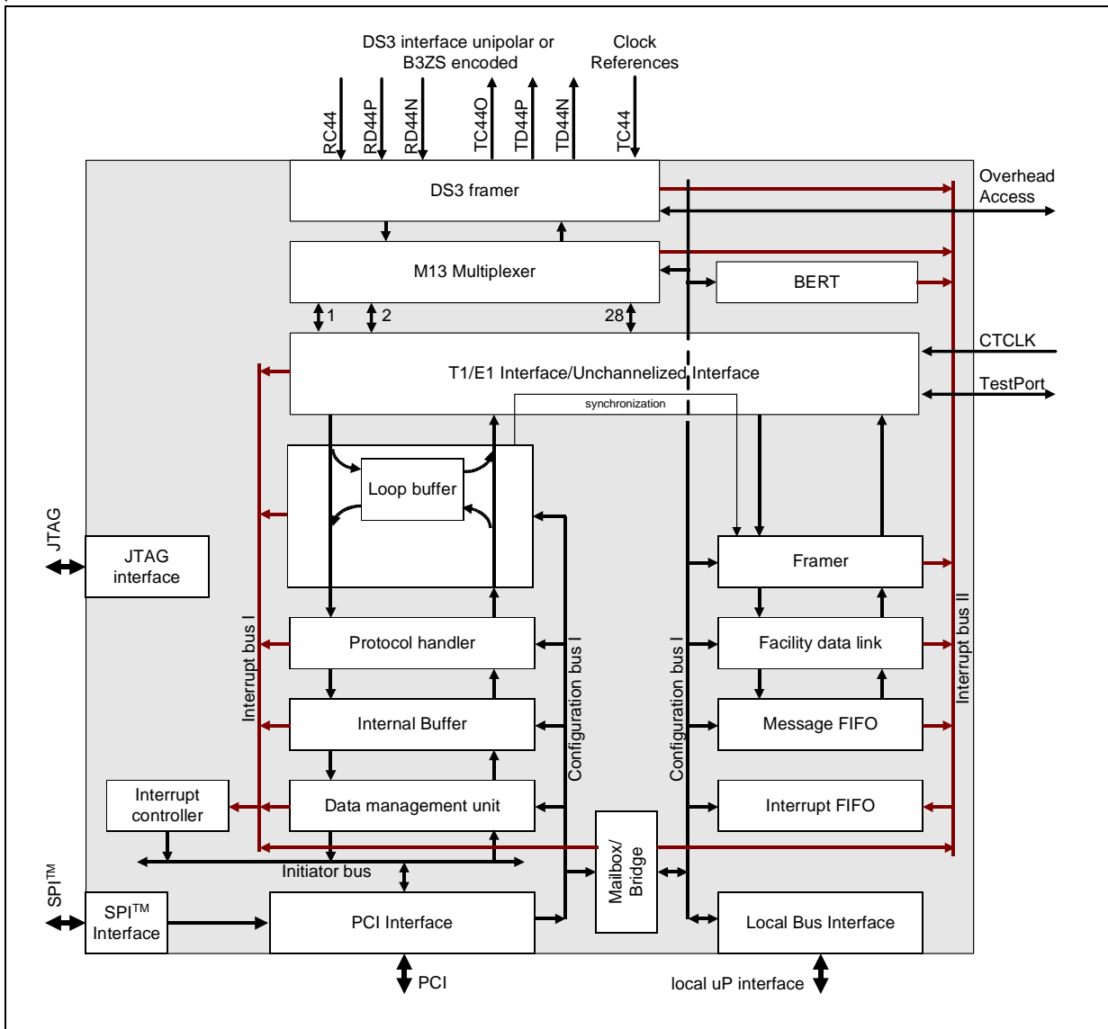
Figure 3-1 TE3-CHATT Block Diagram
