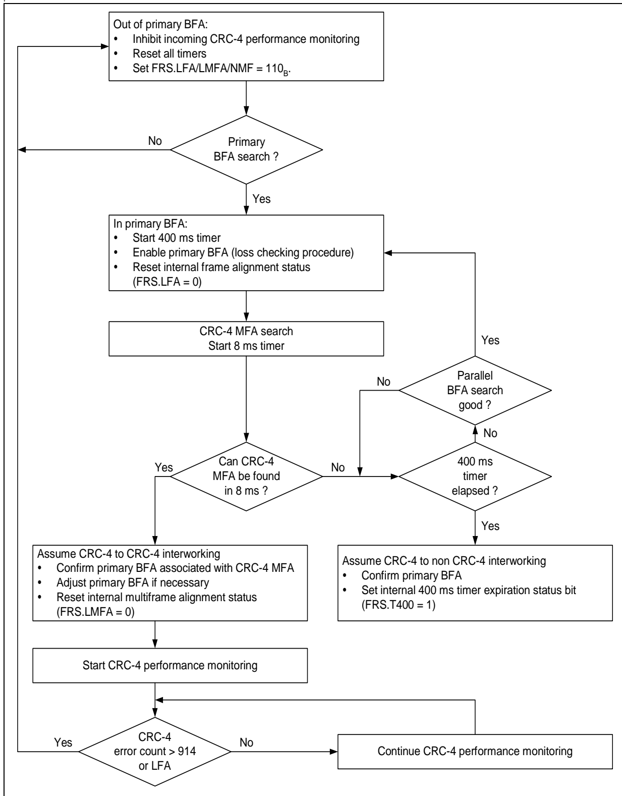
Figure 4-11 CRC-4 Multiframe Alignment Recovery Algorithms
