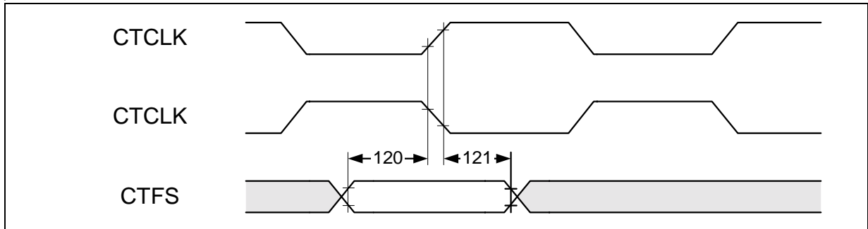
Figure 9-30 T1/E1 Tributary Synchronization Timing
