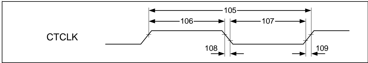
Figure 9-29 T1/E1 Tributary Clock Input Timing
