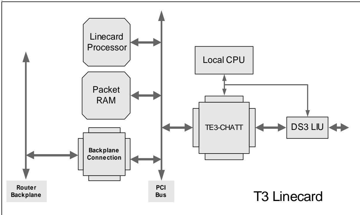
Figure 1-2 System Integration of the TE3-CHATT
