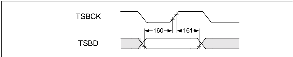
Figure 9-27 DS3 Transmit Stuff Bit Timing
