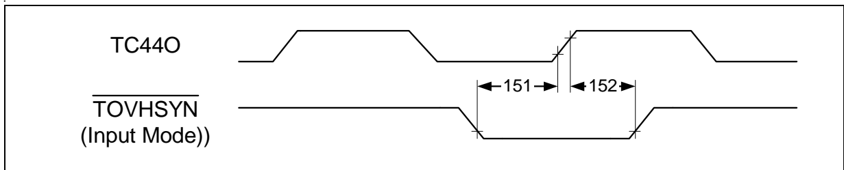
Figure 9-25 DS3 Transmit Overhead Synchronization Timing
