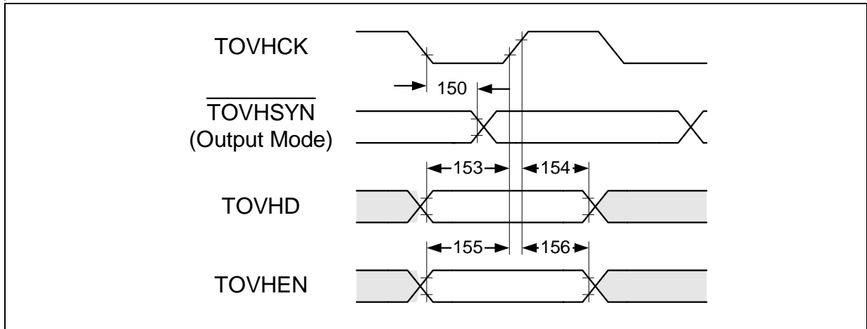
Figure 9-24 DS3 Transmit Overhead Timing
