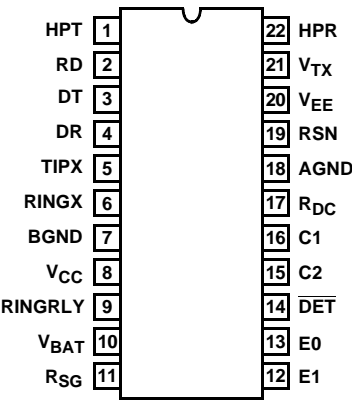
HC5523 (PDIP) TOP VIEW
