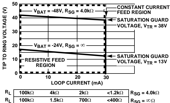
FIGURE 15. V_{TR} vs I_L and R_L
