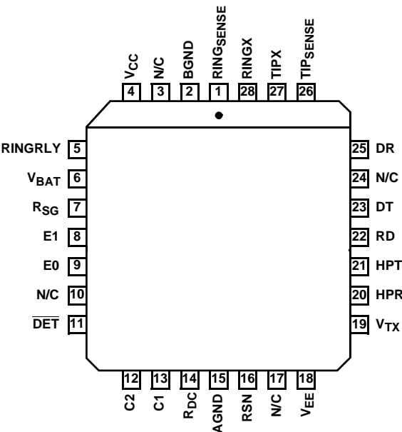
HC5523 (PLCC) TOP VIEW
