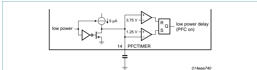
Fig 6. PFC start/stop via PFCTIMER pin
