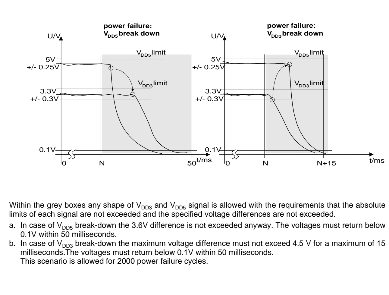
Figure 5-2 Power-Failure scenarios
