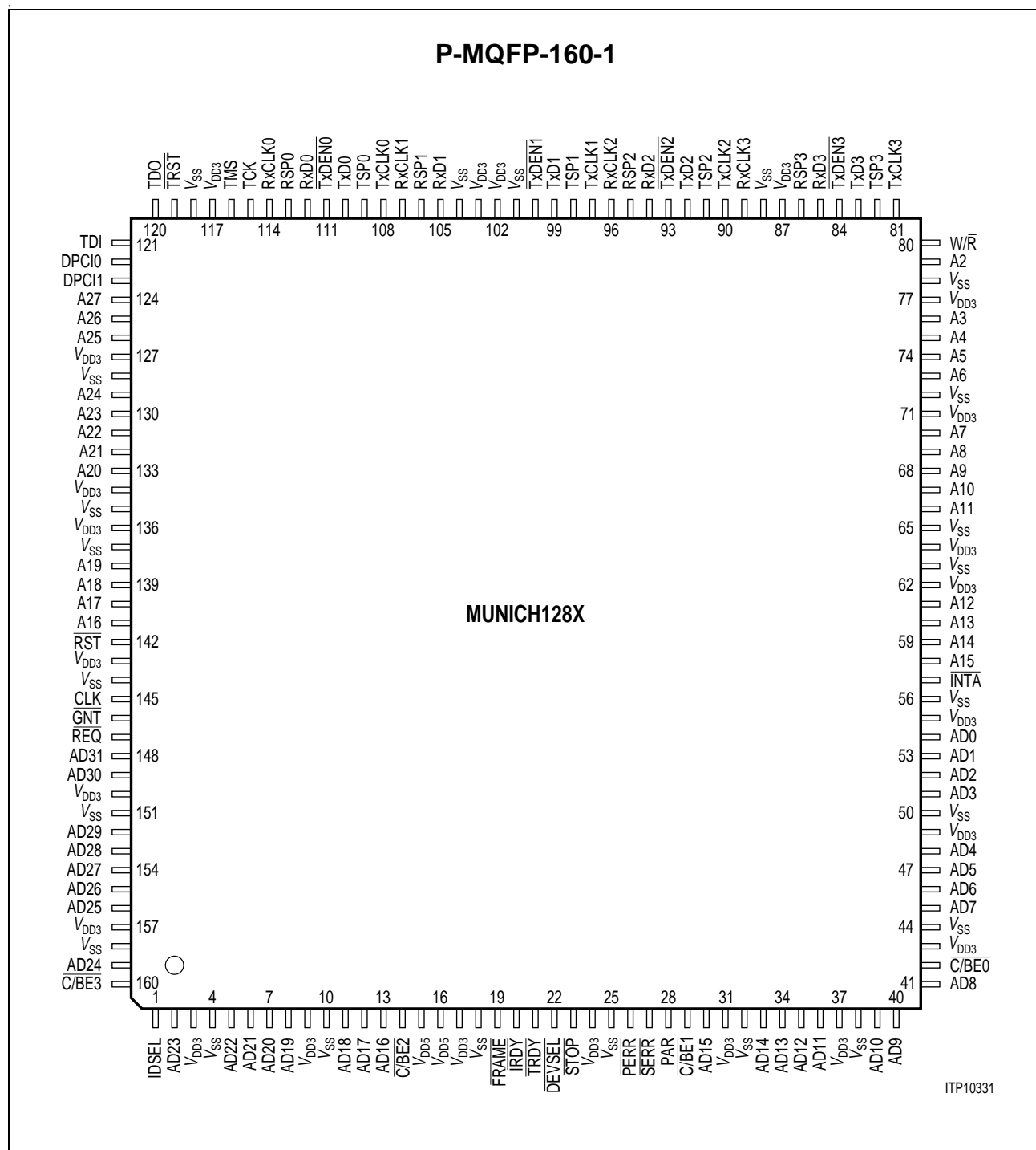
Figure 2-1 Pin Configuration
