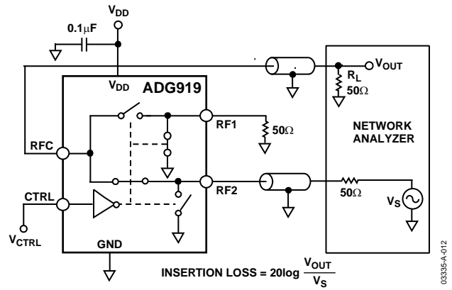
Figure 21. Insertion Loss
