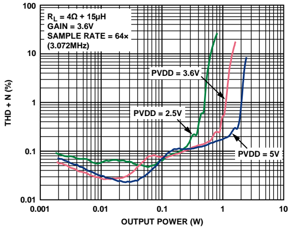
Figure 10. THD + N vs. Output Power into 4Ω, Gain = 3.6 V, f_s = 64\times
