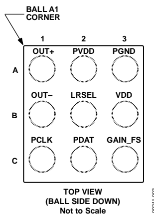
Figure 3. Pin Configuration
