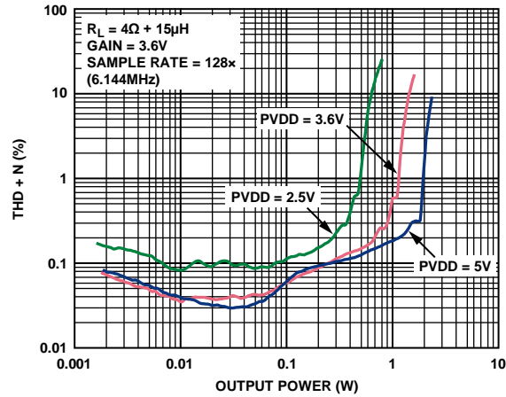
Figure 13. THD + N vs. Output Power into 4Ω, Gain = 3.6 V, f_s = 128\times
