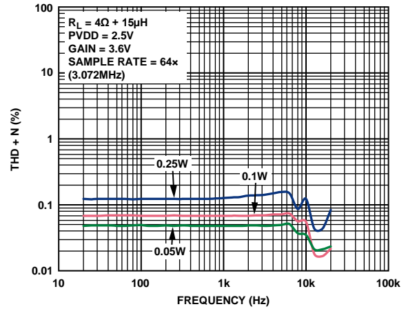
Figure 19. THD + N vs. Frequency, PVDD = 2.5 V, Gain = 3.6 V, R_L = 4\Omega , f_s = 64\times
