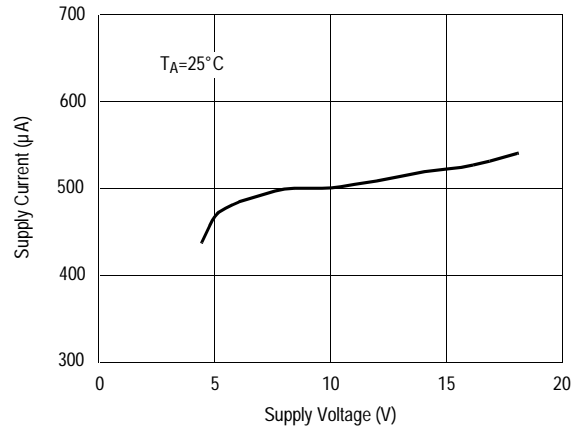
Supply Current per Channel vs Supply Voltage
