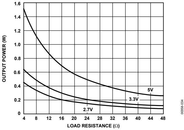
Figure 34. P_{OUTPUT} vs. Load Resistance
