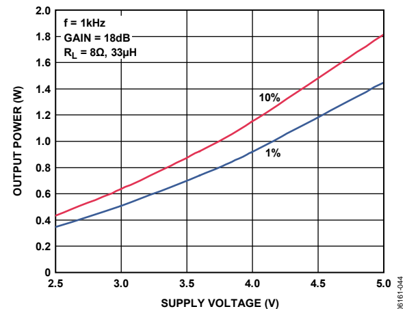
Figure 20. Maximum Output Power vs. Supply Voltage, R_L = 8\ \Omega , A_v = 18\text{ dB}
