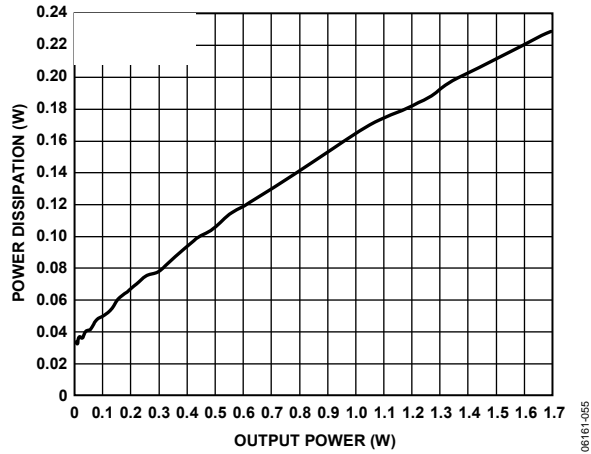
Figure 33. Power Dissipation vs. Output Power into 4 Ω at V_{DD} = 3.6\text{ V}
