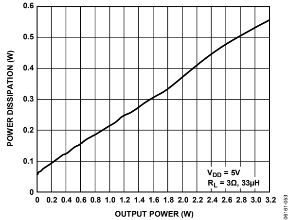
Figure 31. Power Dissipation vs. Output Power into 3 Ω at V_{DD} = 5.0 V
