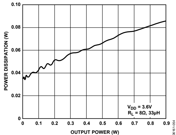
Figure 32. Power Dissipation vs. Output Power into 8 Ω at V_{DD} = 3.6 V
