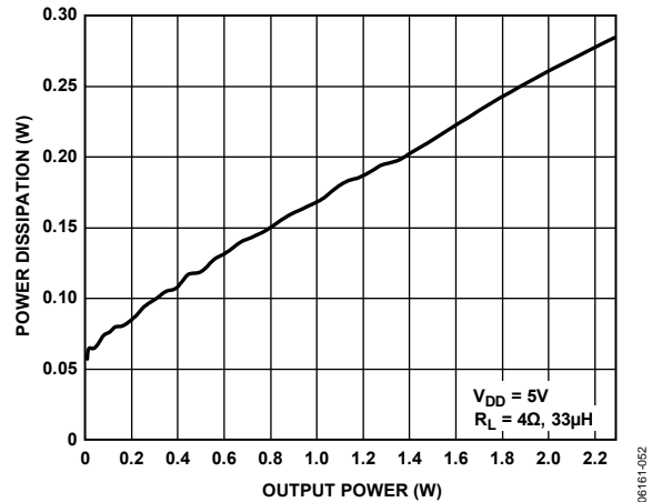
Figure 30. Power Dissipation vs. Output Power into 4 Ω at V_{DD} = 5.0 V
