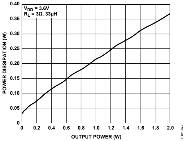
Figure 34. Power Dissipation vs. Output Power into 3 Ω at V_{DD} = 3.6\text{ V}
