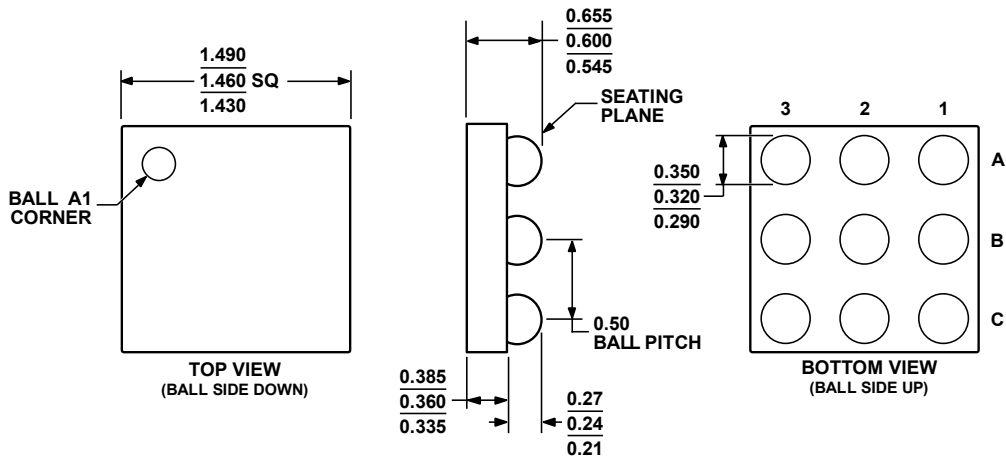
Figure 48. 9-Ball Wafer Level Chip Scale Package [WLCSP] (CB-9-2) Dimensions shown in millimeters
