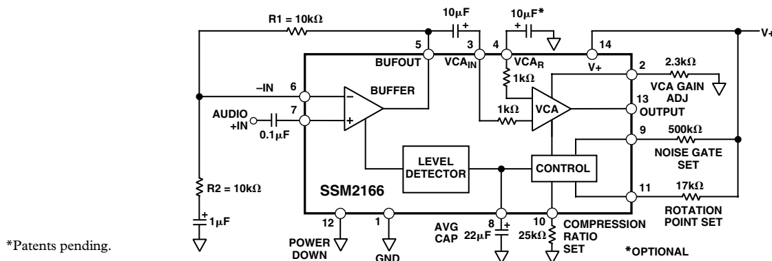
Figure 2. Functional Block Diagram and Typical Speech Application
