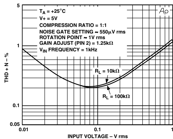
TPC 5. THD + N (%) vs. Input (V rms)
