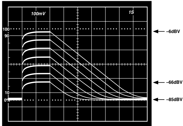
Figure 5b. RMS Level Detector Performance with C_{AVG} = 22 \mu F
