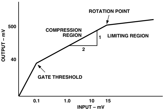
Figure 15. Transfer Characteristic
