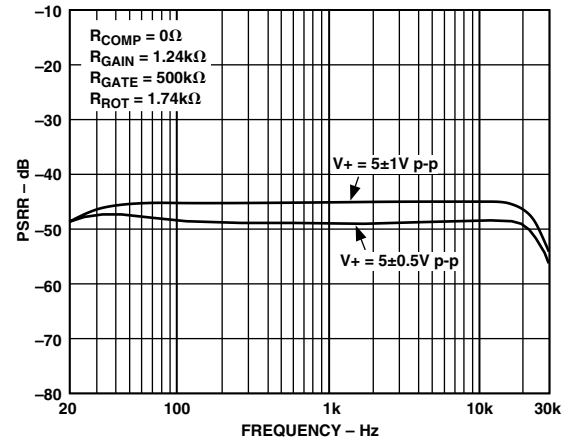
TPC 8c. PSRR vs. Frequency
