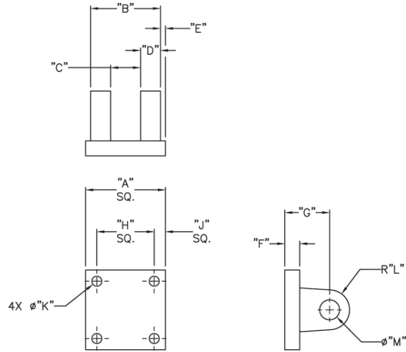
Rear Clevis Dimension Table
