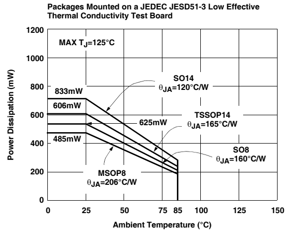
FIGURE 4. PACKAGE POWER DISSIPATION vs AMBIENT TEMPERATURE
