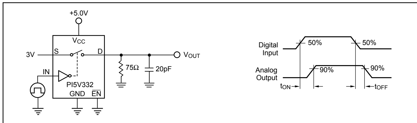
Figure 2. Switching Time
