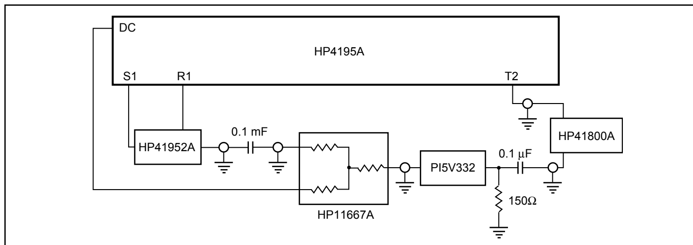
Figure 1. Differential Gain/Phase
