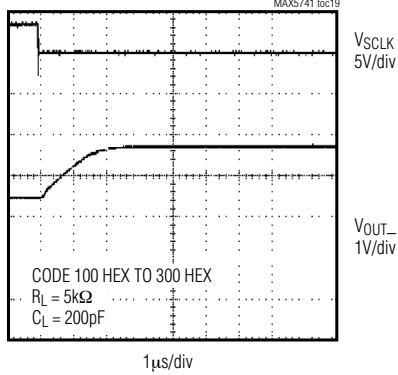
HALF-SCALE SETTLING TIME ( V_{DD} = +3\text{V} ) MAX5741 toc19
