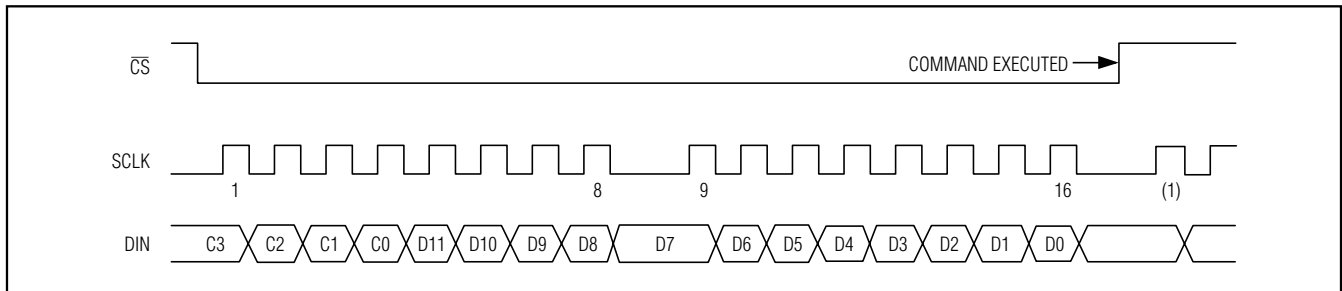
Figure 2. Serial-Interface Signals
