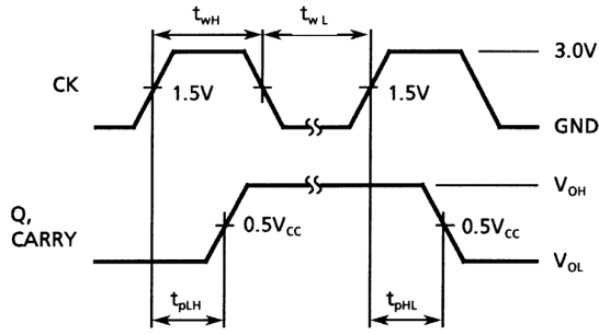
Count Mode
