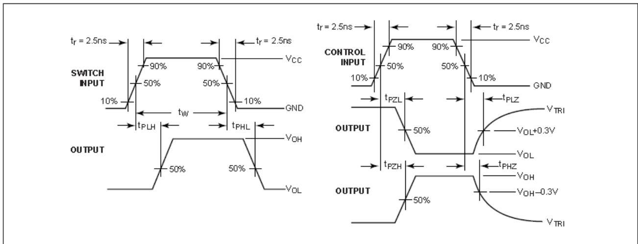
Figure 2. AC Waveforms
