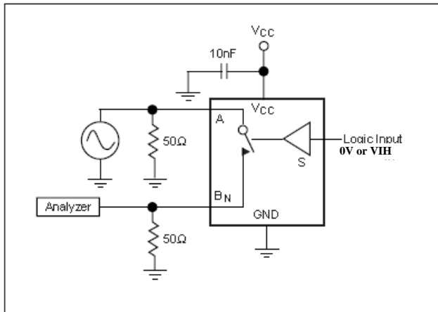
Figure 5. Off Isolation
