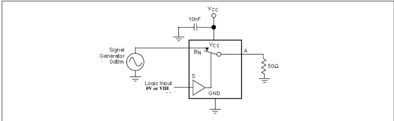
Figure 9. Bandwidth
