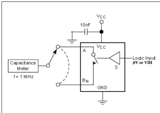
Figure 7. Channel Off Capacitance
