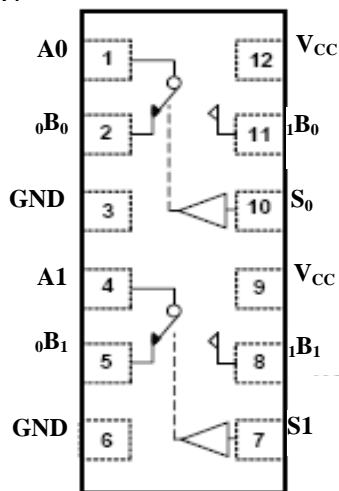
TDFN-12
