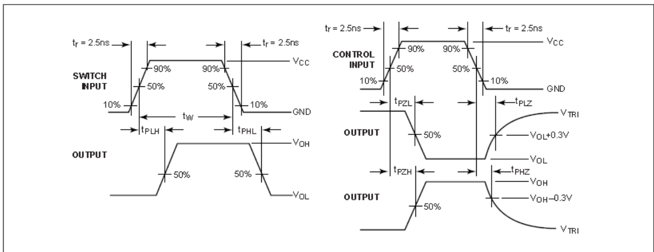
Figure 2. AC Waveforms
