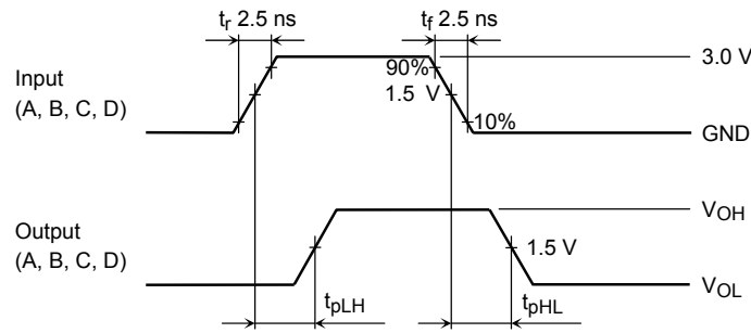
Figure 2 t_{pLH} , t_{pHL}
