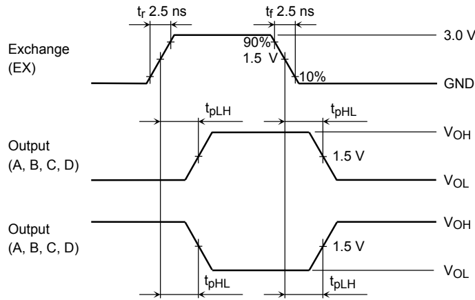
Figure 3 t_{pLH} , t_{pHL}
