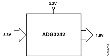
Figure 33. 3.3 V to 1.8 V Voltage Translation, \overline{SEL} = 0\text{ V}
