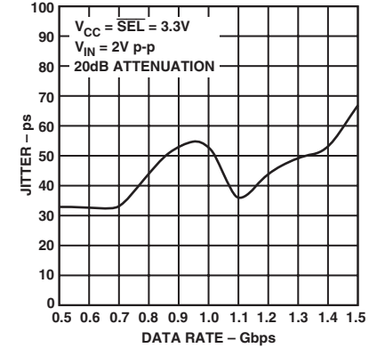
TPC 18. Jitter vs. Data Rate; PRBS 31
