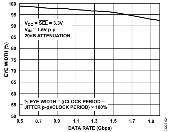
Figure 21. Eye Width vs. Data Rate; PRBS 31
