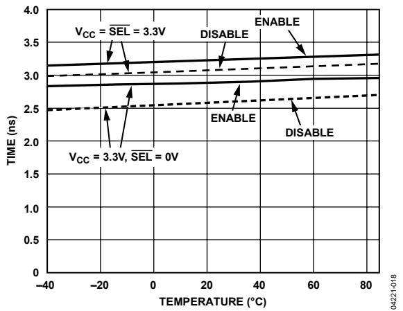
Figure 18. Enable/Disable Time vs. Temperature
