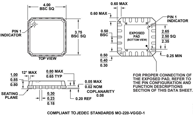
Figure 38. 20-Lead Lead Frame Chip Scale Package [LFCSP_VQ] 4 mm x 4 mm Body, Very Thin Quad (CP-20-4) Dimensions shown in millimeters
