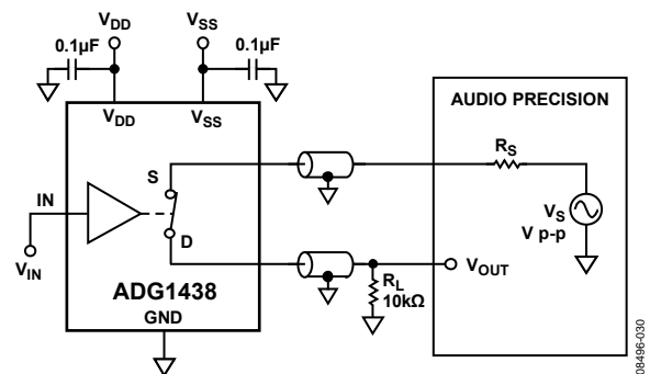
Figure 36. THD + Noise
