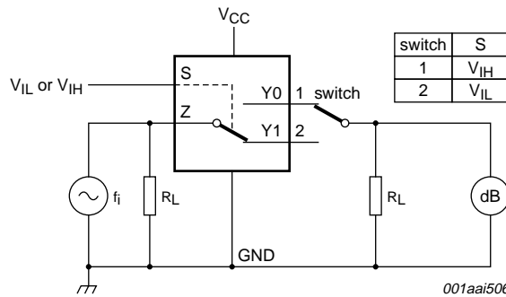
Fig 8. Test circuit for measuring isolation (OFF-state)
