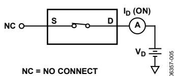
Figure 20. On Leakage
