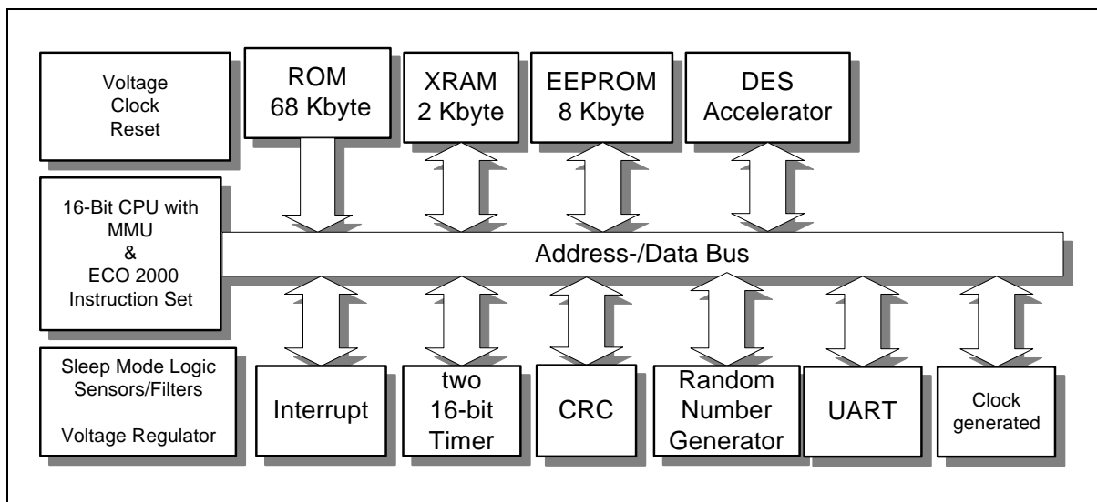
Figure 2: Block Diagram SLE 66C86PE
