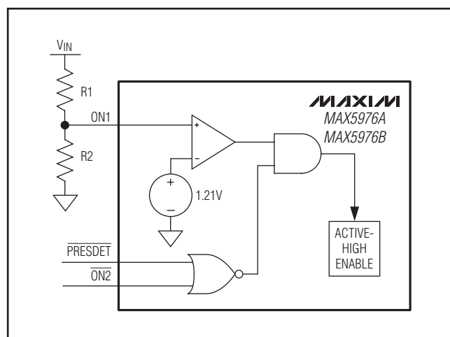
Figure 1. Undervoltage Threshold Setting
