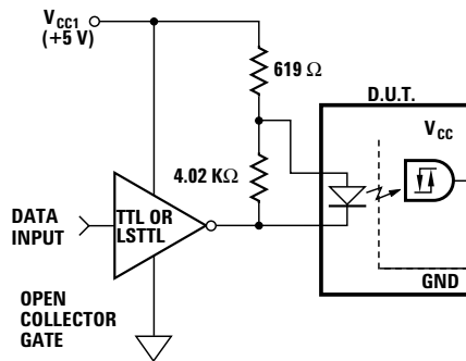
Figure 12. Series LED Drive with Open Collector Gate (4.02 kOhm Resistor Shunts I_{OH} from the LED).
