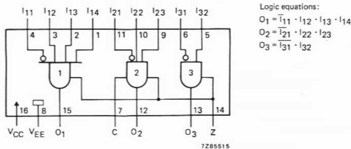
Fig. 1 Logic diagram.
