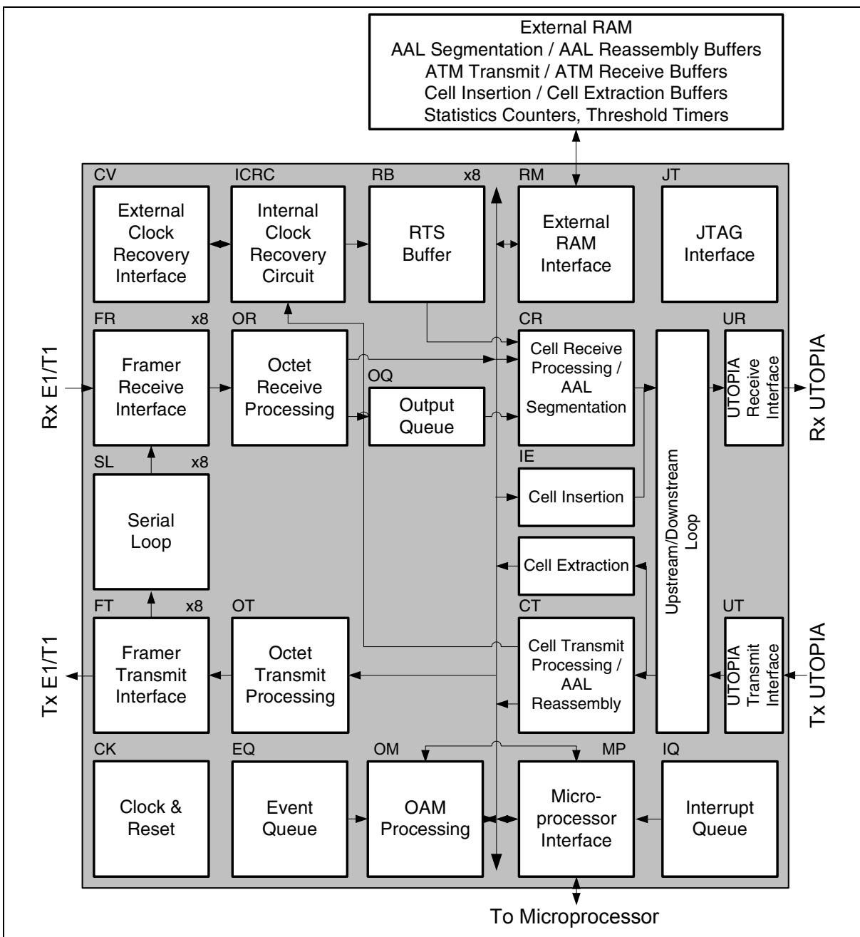
Figure 6 Block Diagram
