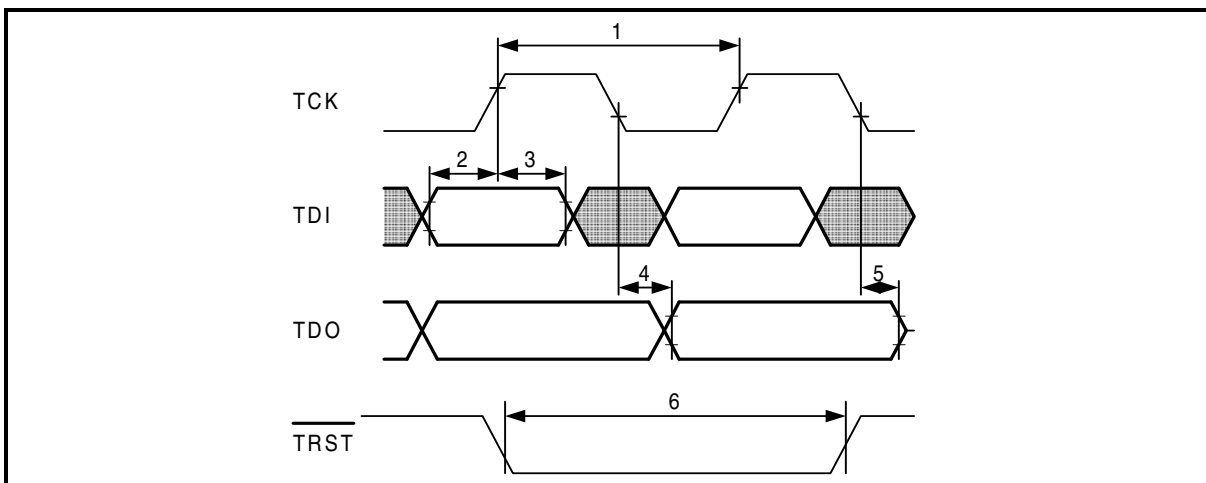
Figure 72 Boundary-Scan Test Interface Timing Diagram
