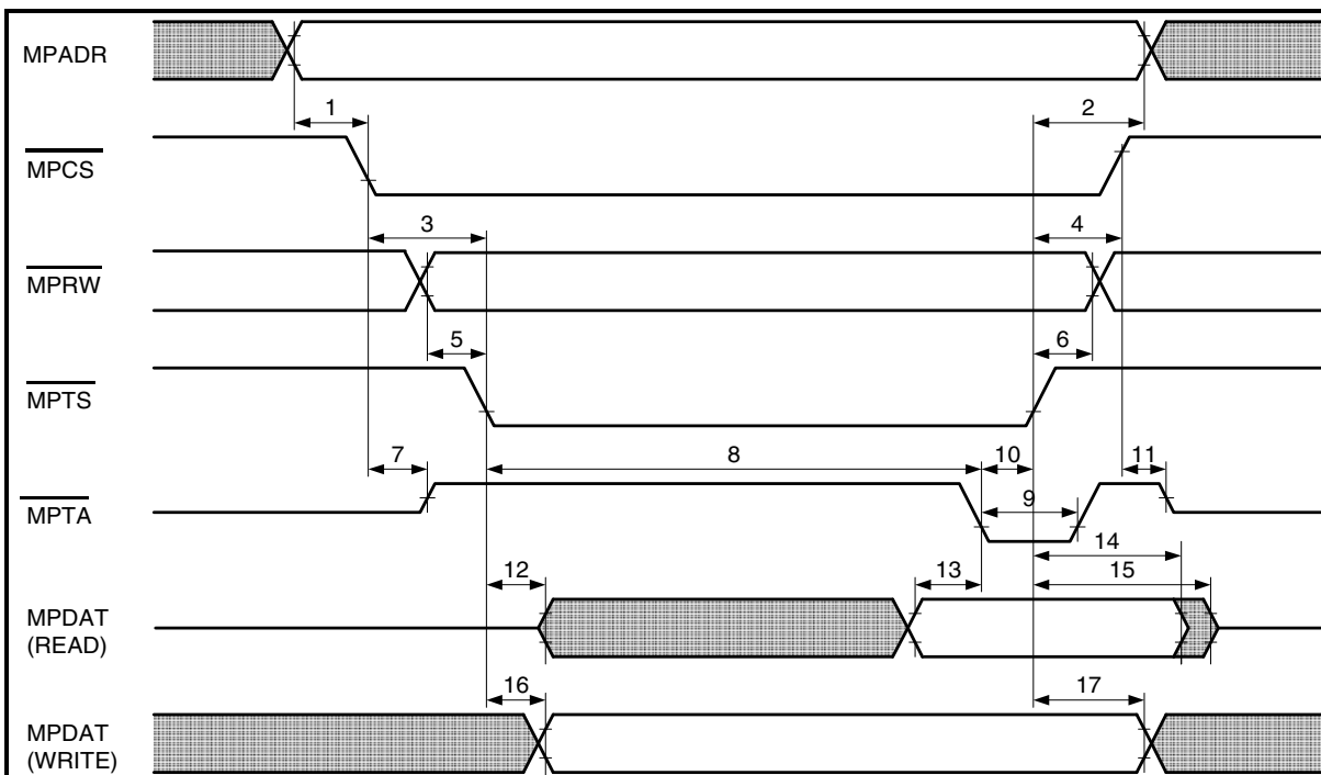
Figure 70 Motorola Mode Timing Diagram
