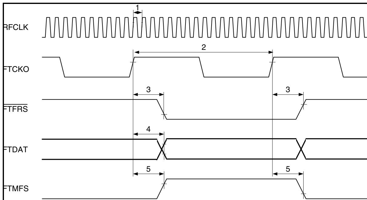
Figure 60 Framer Transmit Interface Timing in GIM
