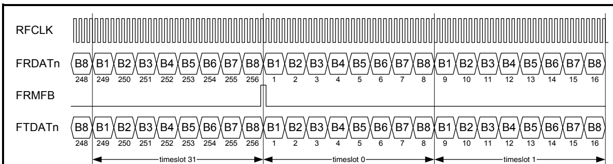
Figure 27 Framer Interface in SYM8 E1
