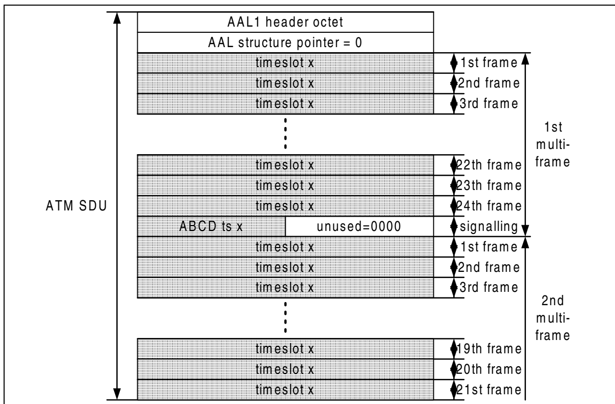
Example Multiframe Structure for 1x64 Kbit/s DS1 with CAS
