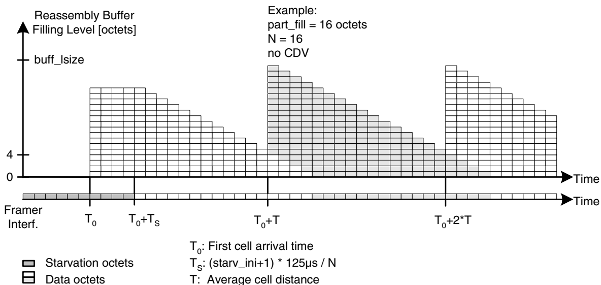
Figure 15 Reassembly Buffer Initialization: No CDV
