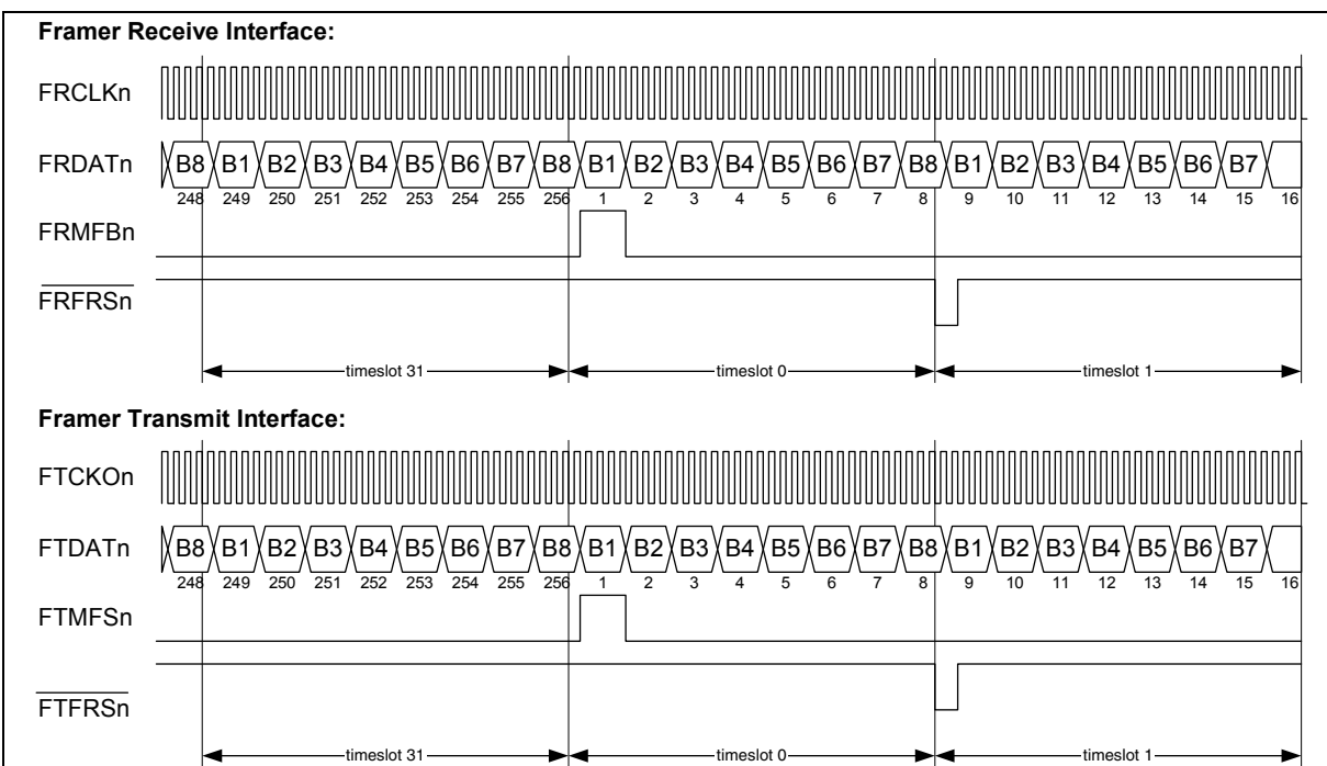
Figure 23 Framer Interface in FAM
