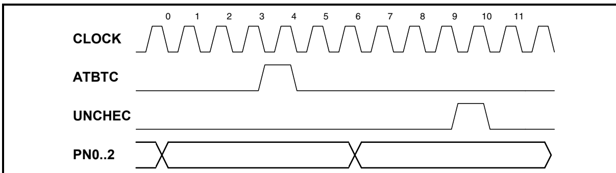
Figure 31 IMA Interface Protocol
