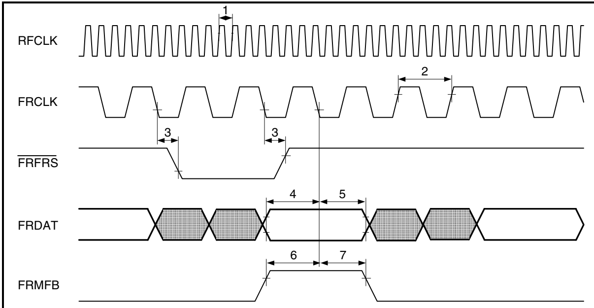
Figure 57 Framer Receive Interface Timing in FAM
