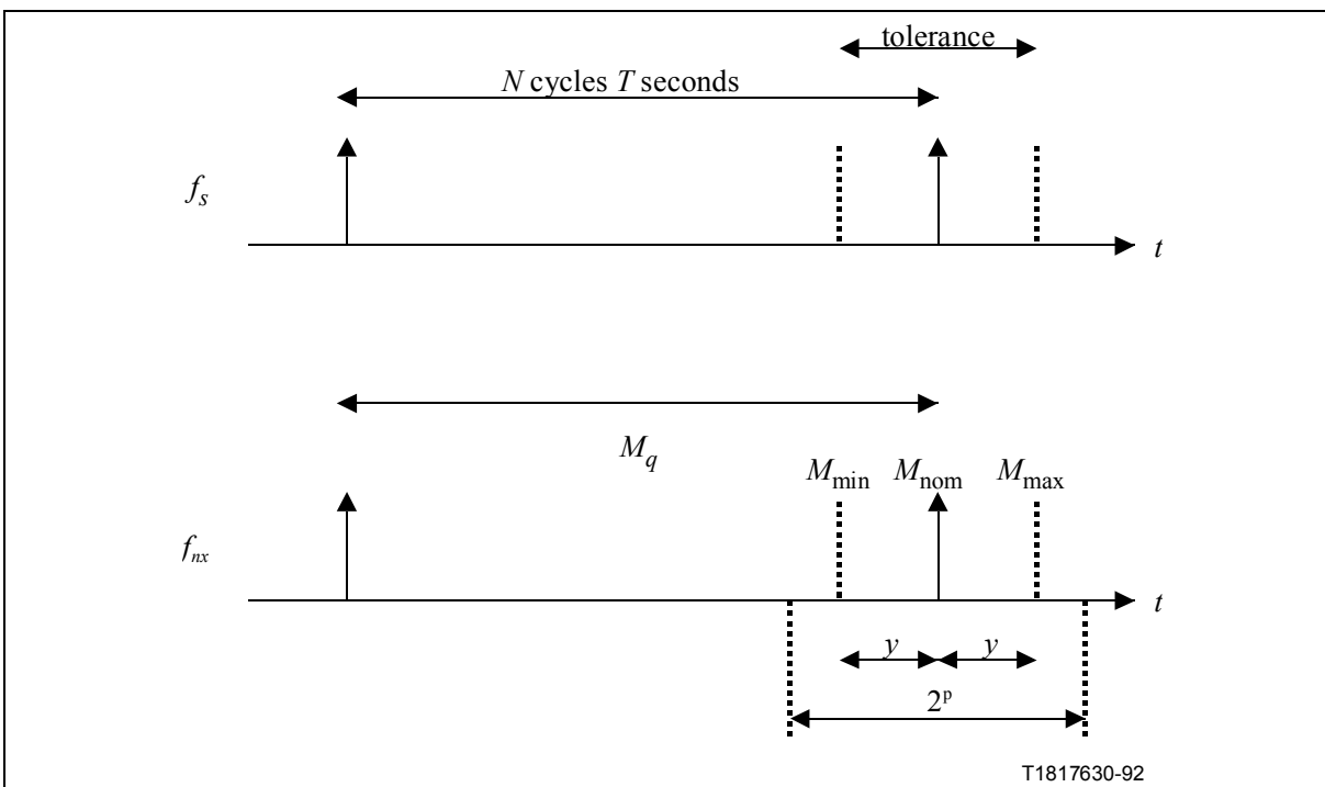
Figure 76 The Concept of Synchronous Residual Time Stamp (SRTS) (Fig. 5/ I.363.1)
