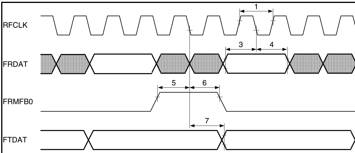
Figure 62 Framer Interface Timing in SYM 8.192 MHz
