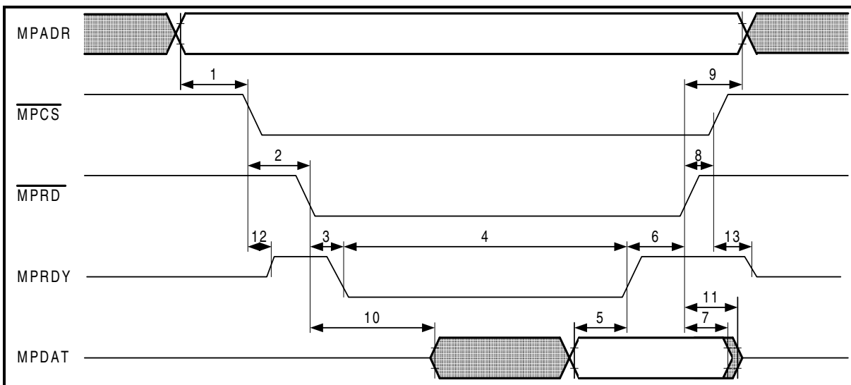
Figure 69 Intel Mode Read Cycle Timing Diagram
