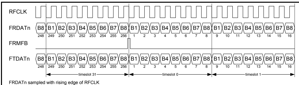
Figure 26 Framer Interface in SYM2 E1
