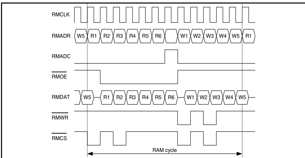
Figure 35 RAM Interface Protocol
