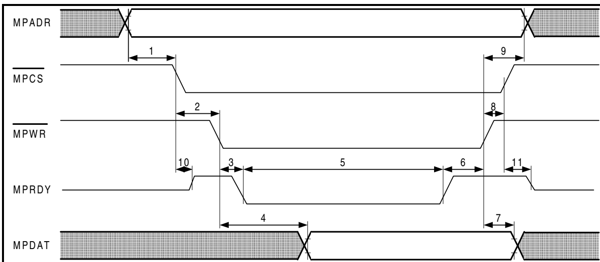
Figure 68 Intel Mode Write Cycle Timing Diagram
