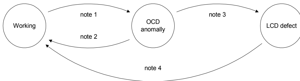
Figure 7 Cell delineation state diagram (Figure 5/I.432.1)
