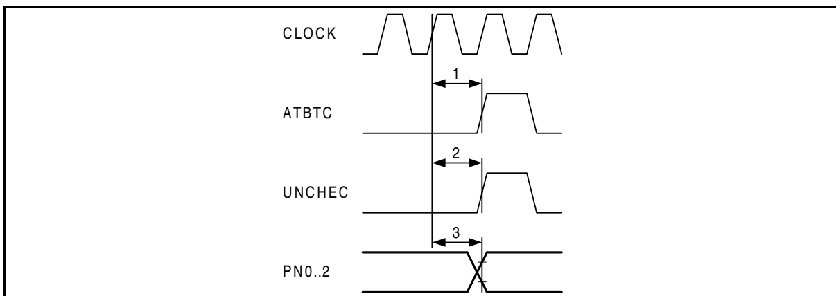
Figure 66 Timing of the IMA Interface
