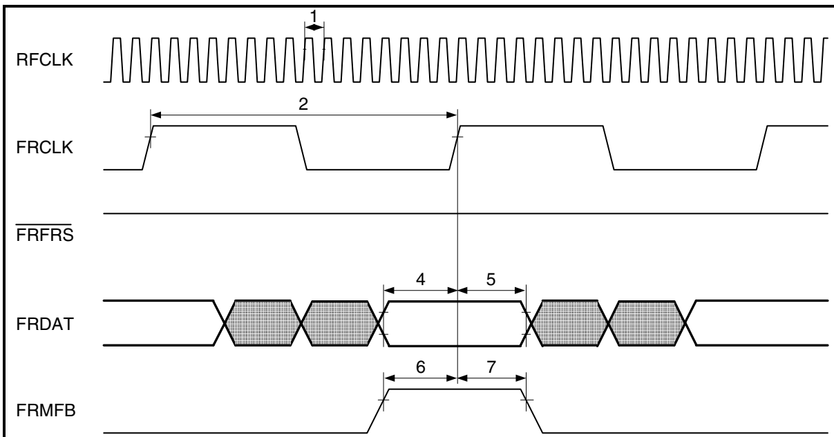
Figure 59 Framer Receive Interface Timing in GIM
