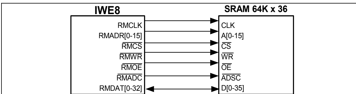
Figure 34 External RAM Connection
