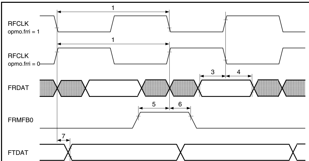
Figure 61 Framer Interface Timing for SYM 2.048 MHz
