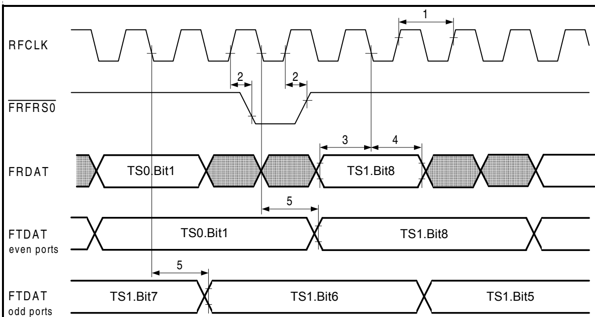
Figure 63 Framers Interface Timing in EC Mode
