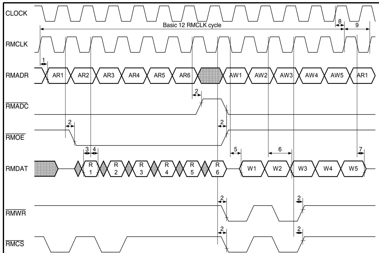
Figure 71 RAM Interface Timing Diagram
