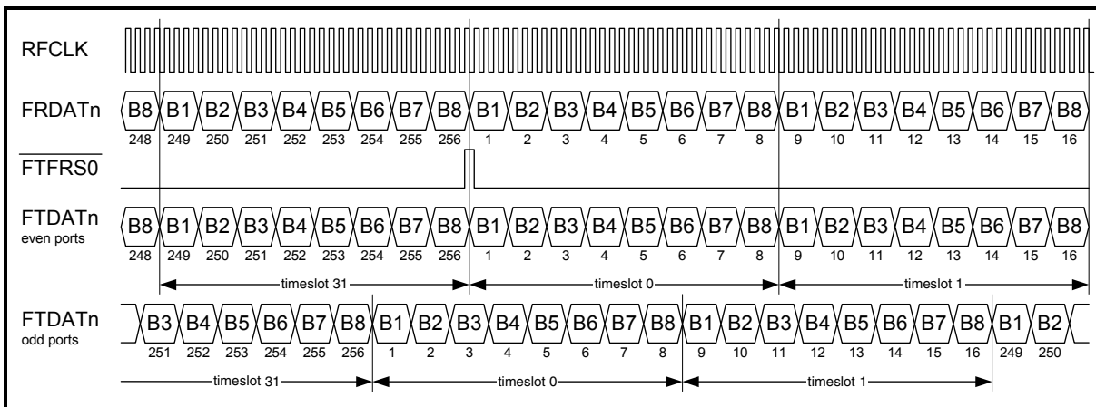
Figure 28 Framer Interface in EC Mode
