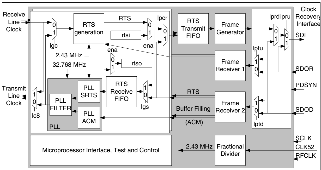
Figure 19 Block Diagram of the ICRC
