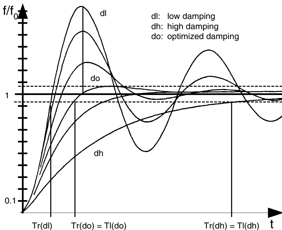
Figure 21 Influence of Damping on Lock in Time
