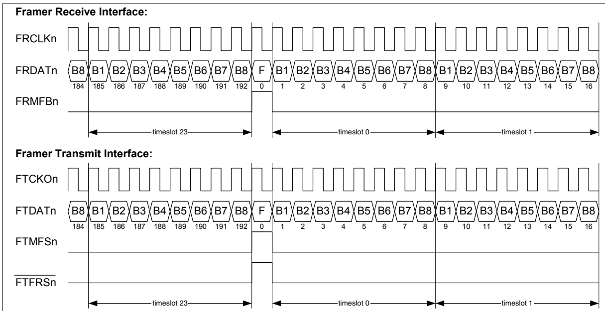
Figure 24 Framer Interface in GIM T1
