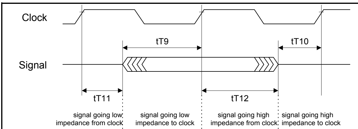
Figure 65 Tri-state timing (multi-PHY, multiple devices only)
