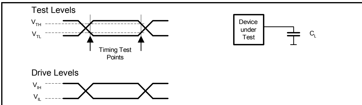
Figure 55 Input/Output Waveforms for AC Measurements
