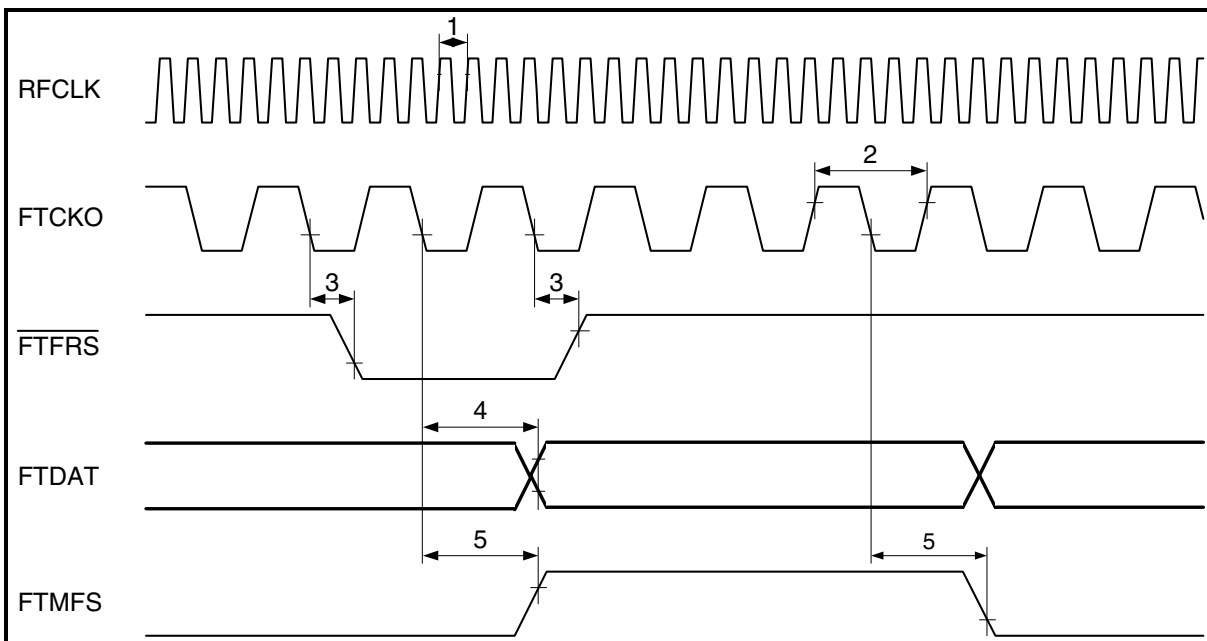
Figure 58 Framer Transmit Interface Timing in FAM
