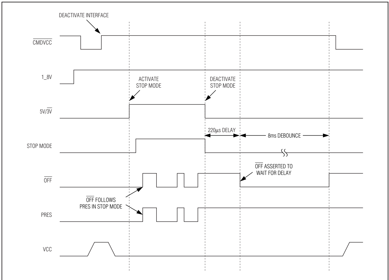
Figure 8. Stop-Mode Sequence
