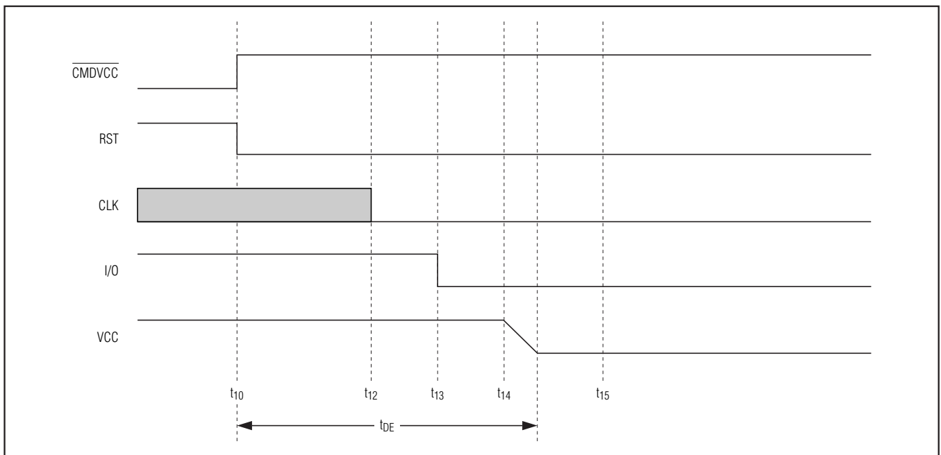
Figure 5. Deactivation Sequence
