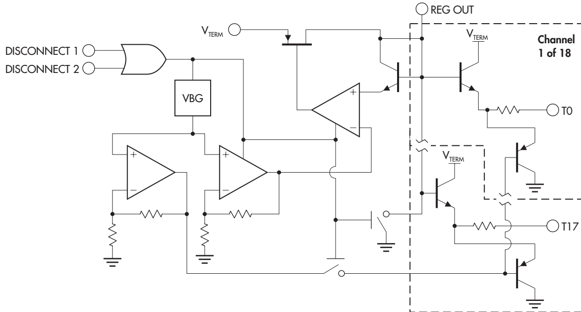
FIGURE 1 — LX5205 BLOCK DIAGRAM
