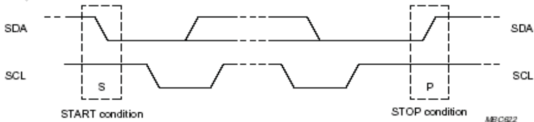
Fig.6 START and STOP conditions.
