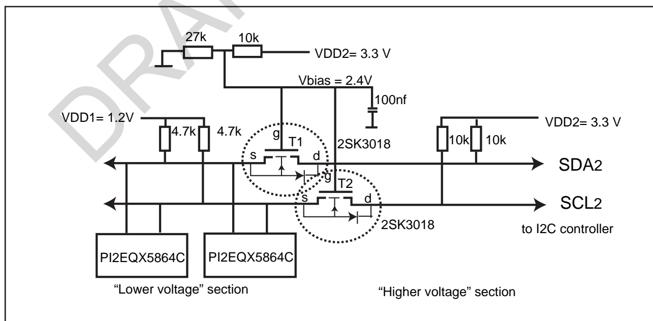
Figure 2. Bi-directional Level Shifter Circuit
