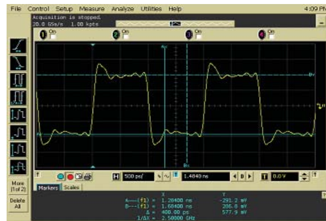
-3.5 dB (Dx = 010)
