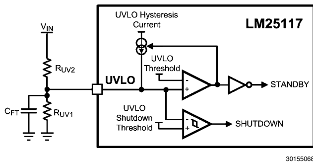
FIGURE 6. UVLO Configuration
