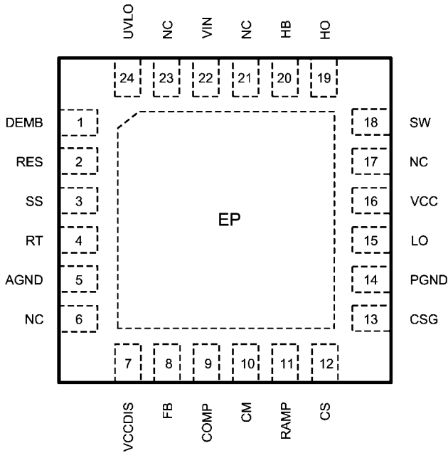
Top View LLP-24 (4mmx4mm)
