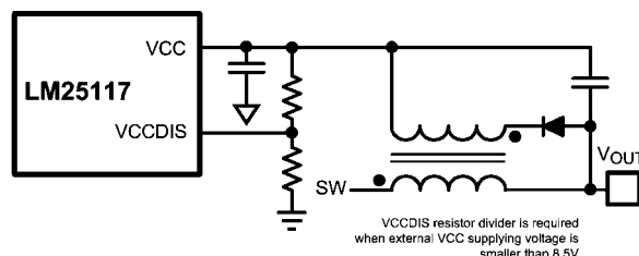
FIGURE 4. External VCC Supply for V_{OUT} < 5V
