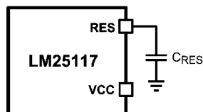
(a) Hiccup Mode Current Limit
