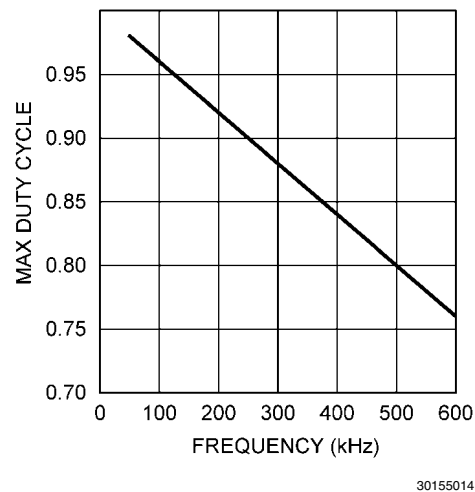
FIGURE 15. Maximum Duty Cycle vs Switching Frequency
