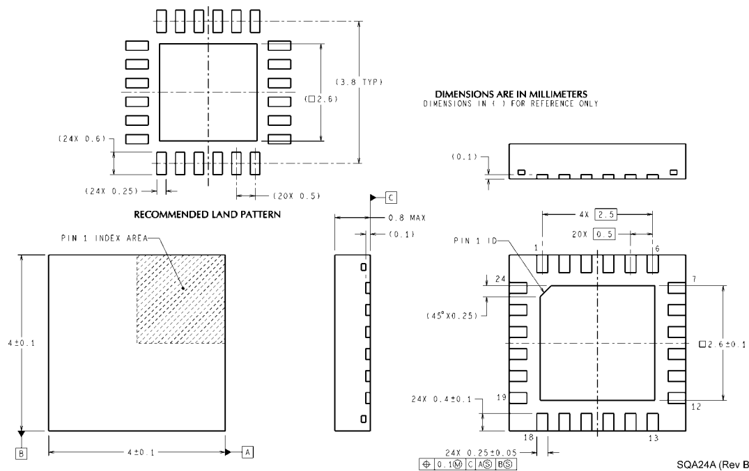
24 Pin LLP NS Package Number SQA24A
