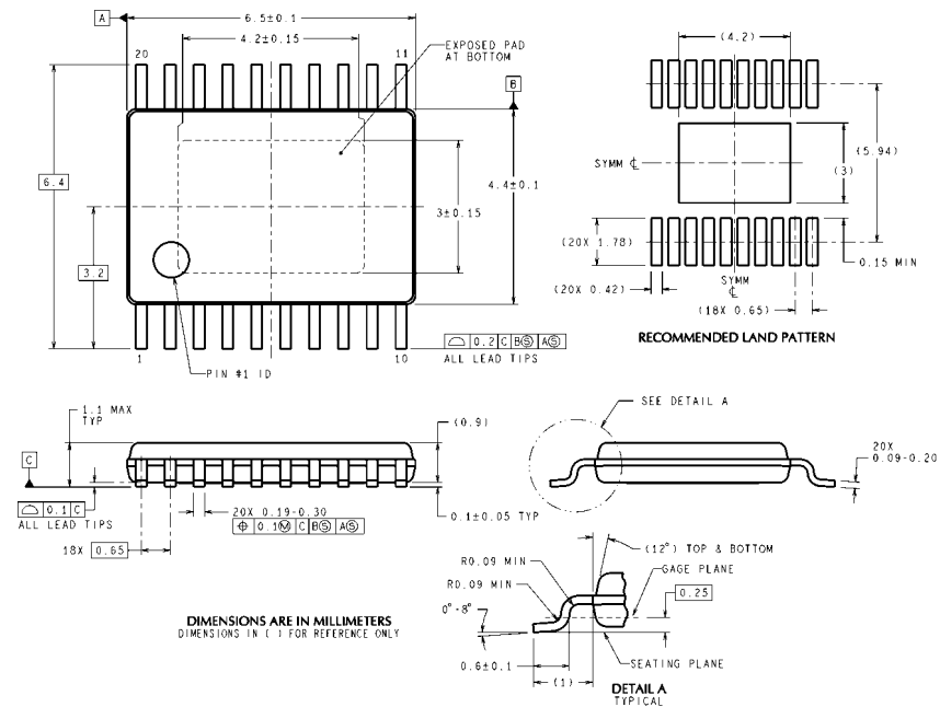
20 Pin TSSOP with Exposed Pad NS Package Number MXA20A
