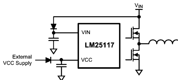
FIGURE 2. VIN Configuration for V_{IN} < V_{VCC}
