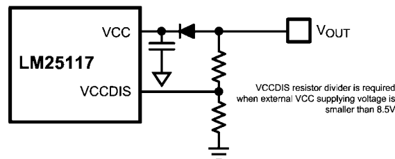
FIGURE 3. External VCC Supply for 5V < V_{OUT} < 14.5V
