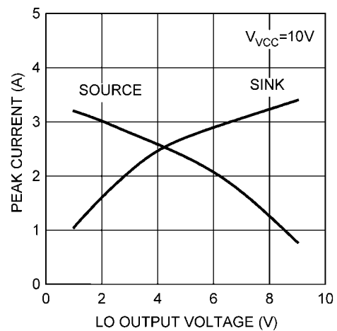
LO Peak Driver Current vs Output Voltage
