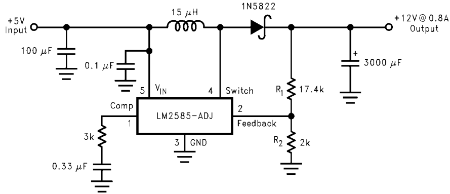
FIGURE 38. Boost Regulator
