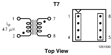
FIGURE 15. Coilcraft S6000-A
