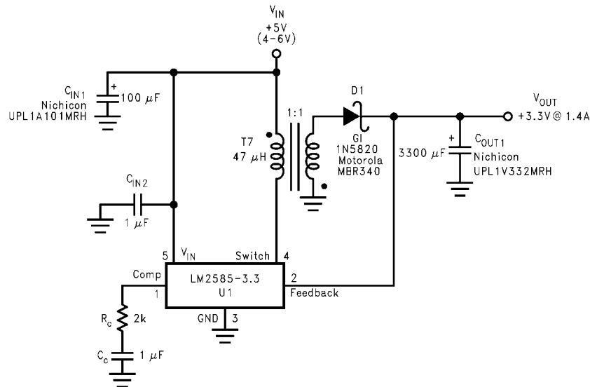
FIGURE 7. Single-Output Flyback Regulator
