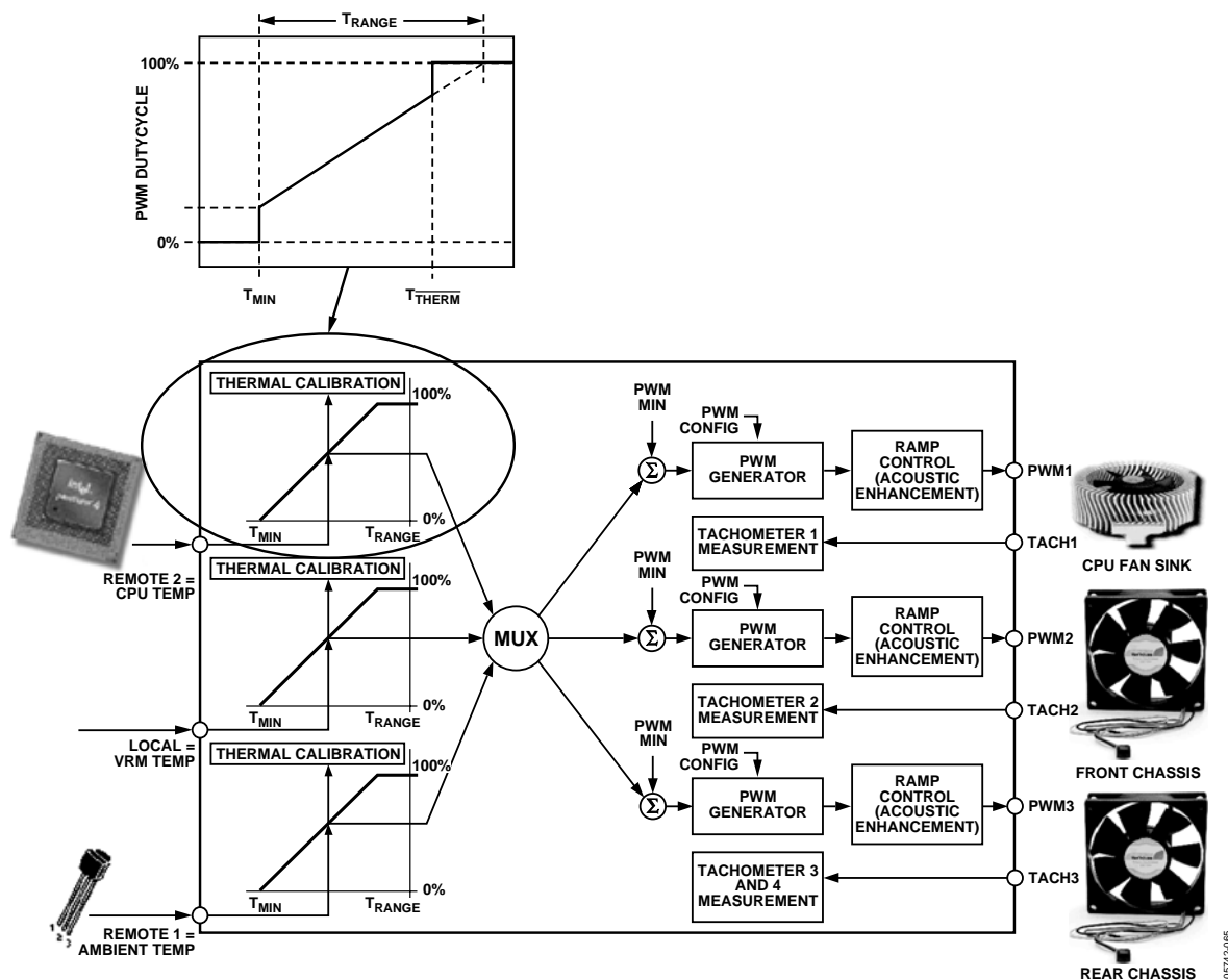
Figure 64. How T_{\text{THERM}} Relates to Automatic Fan Control
