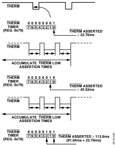
Figure 32. Understanding the \overline{THERM} Timer
