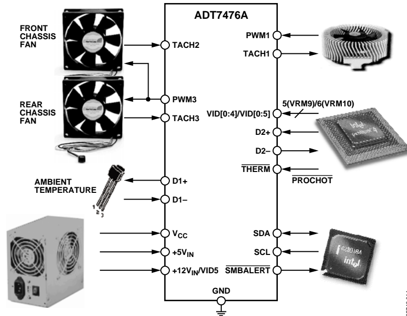
Figure 13. ADT7476A Configuration
