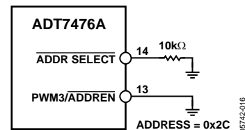
Figure 15. SMBus Address = 0x2C (Pin 14 = 0)
