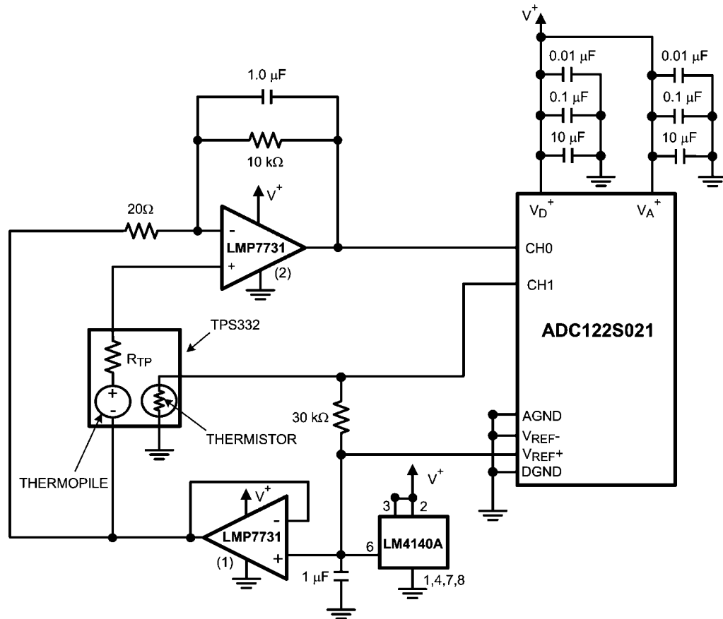
FIGURE 8. Thermopile Amplifier
