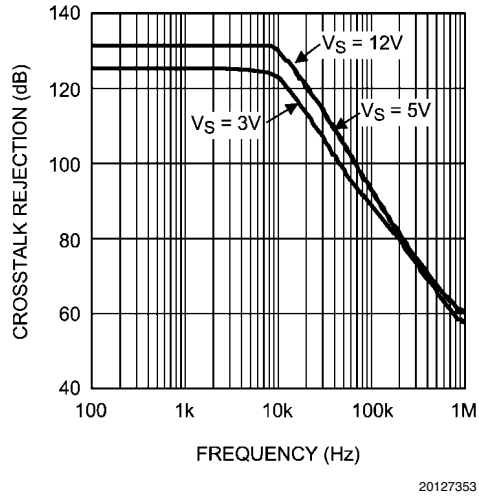
Crosstalk Rejection Ratio vs. Frequency (LMP7702/LMP7704)
