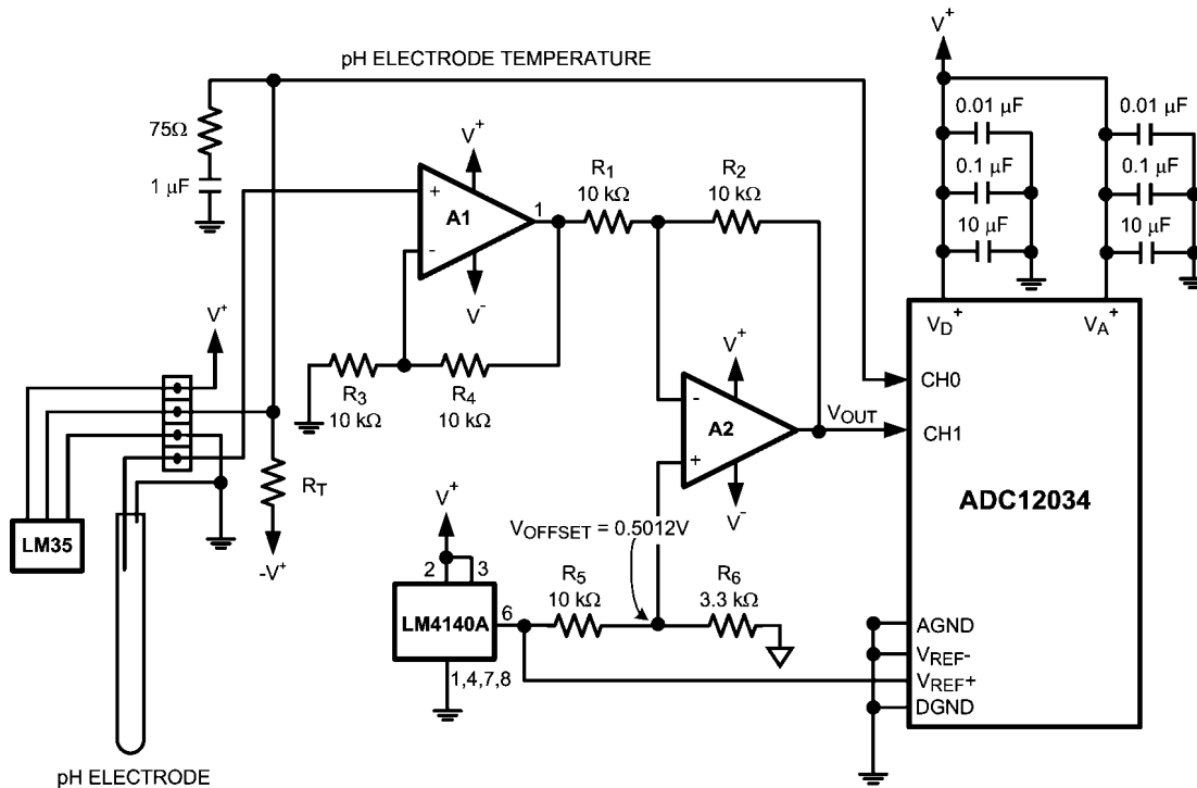
FIGURE 12. pH Measurement Circuit
