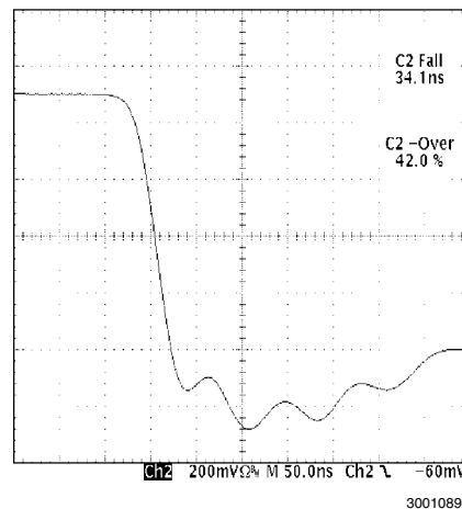
FIGURE 18. Fall Time
