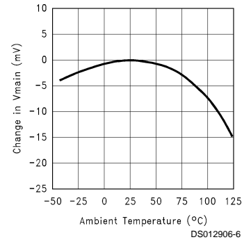
Normalized Main Output Voltage vs Temperature
