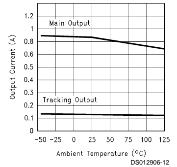
Output Short Circuit Current vs Temperature
