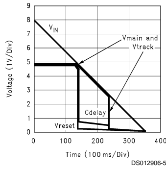
Turn-OFF Characteristic
