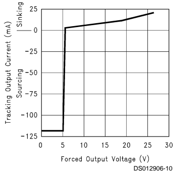
Tracking Output Short Circuit Current
