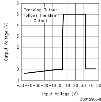
Main Output Voltage at Input Voltage Extremes
