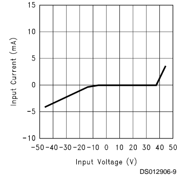
Input Current vs Input Voltage (Regulators OFF)
