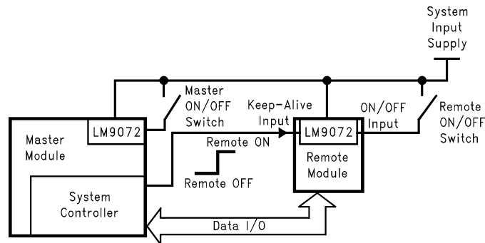
FIGURE 3. Remote ON/OFF Control
