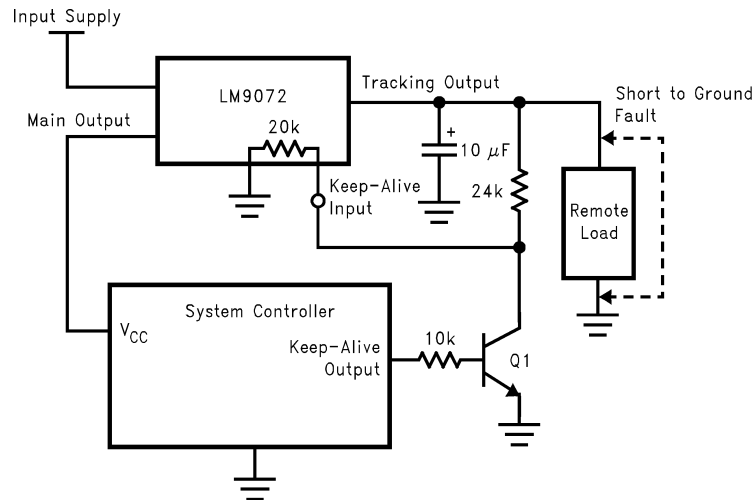
FIGURE 6. Safety Latch-Off
