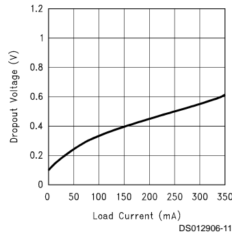
Main Regulator Dropout Voltage vs Load Current
