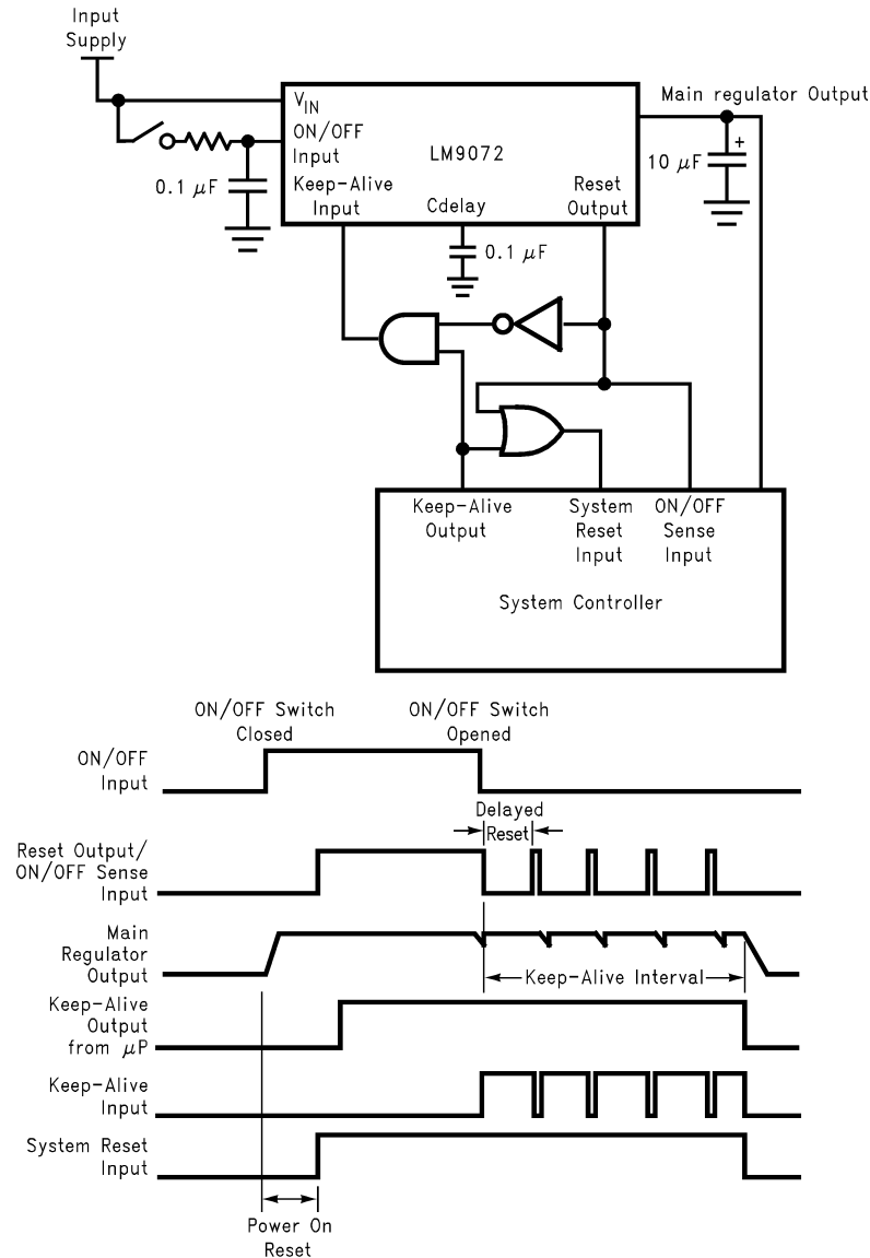
FIGURE 5. Simple Logic Configuration to Provide ON/OFF Sensing
