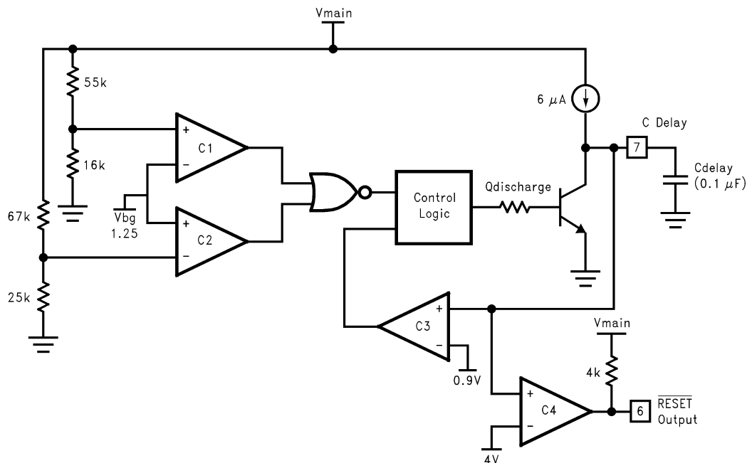
FIGURE 2. Reset Generator
