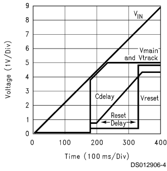
Turn-ON Characteristic
