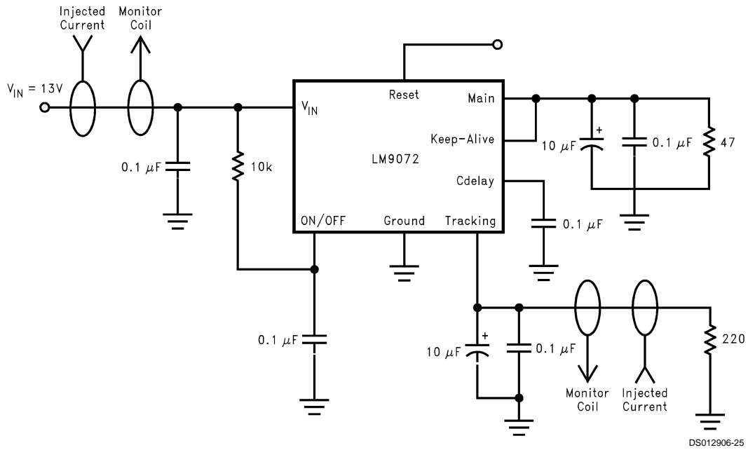
FIGURE 9. Bulk Current Injection Test Configuration
