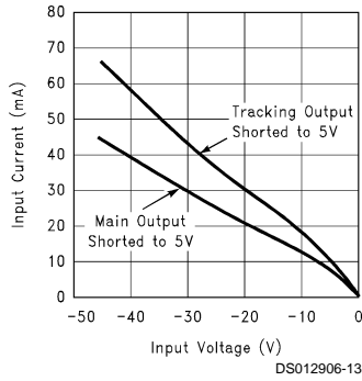
Reverse Battery Input Current
