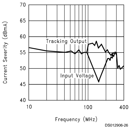
BCI Susceptibility, Modulation 1 (CW)
