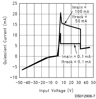
Quiescent Input Current vs Input Voltage
