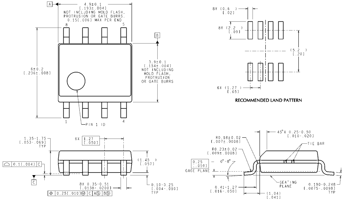
CONTROLLING DIMENSION IS MILLIMETER VALUES IN [ ] ARE INCHES DIMENSIONS IN ( ) FOR REFERENCE ONLY 8-Lead (0.150" Wide) Molded SO Package NS Package Number M08A
