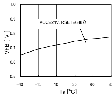
Fig.6 VSET Constant electric current characteristic
