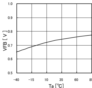
Fig.11 Open detection temperature characteristic
