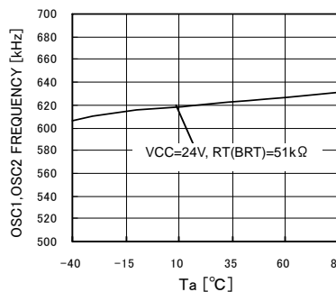
Fig.3 OSC1, OSC2 Temperature re characteristic
