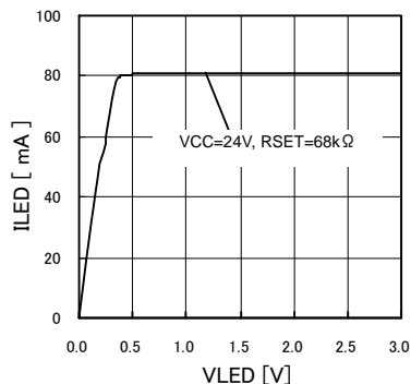
Fig.4 ILED depending on VLED
