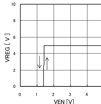
Fig.9 EN Threshold voltage
