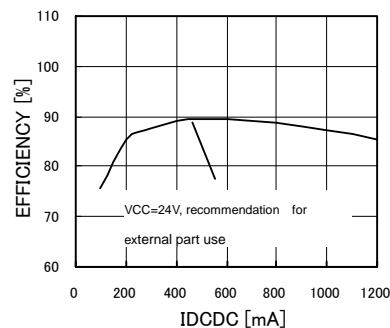
Fig.12 Efficiency
