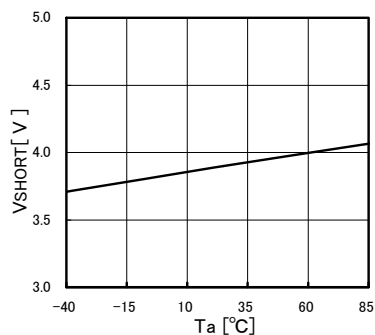
Fig.10 Short detection temperature characteristic
