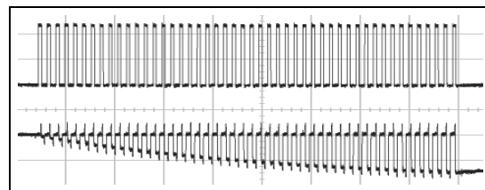
Figure 2-3 Vcs - Correct
