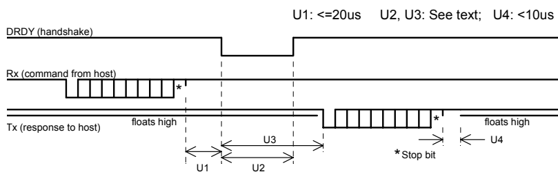
Figure 3-4 UART Timing
