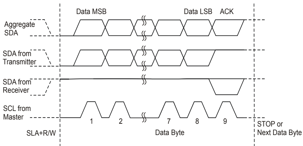
Figure 5-6. Packet Transmission
