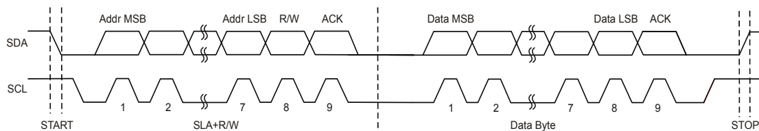
Figure 5-6. Packet Transmission
