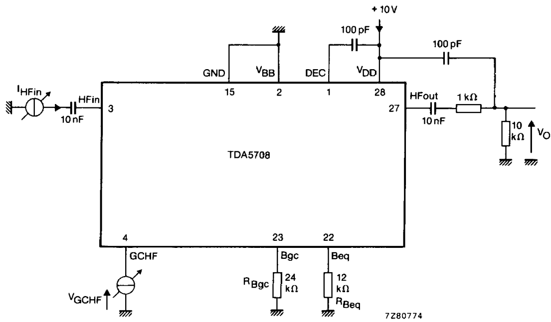
Fig. 13 Test circuit for HF part; a.c. characteristics.
