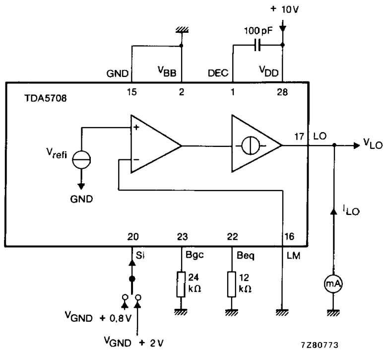
Fig. 12 Test circuit for V_{LO} and I_{LO} .
