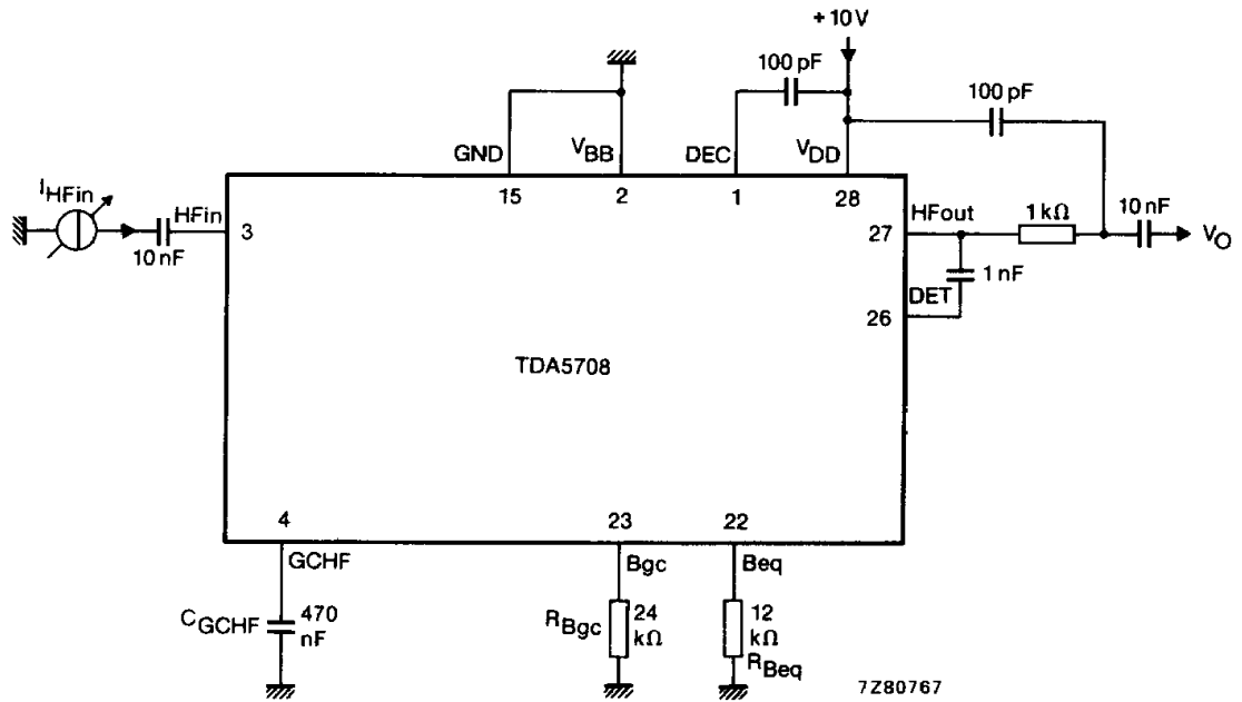
Fig. 6 Test circuit for HF-part; closed-loop condition.
