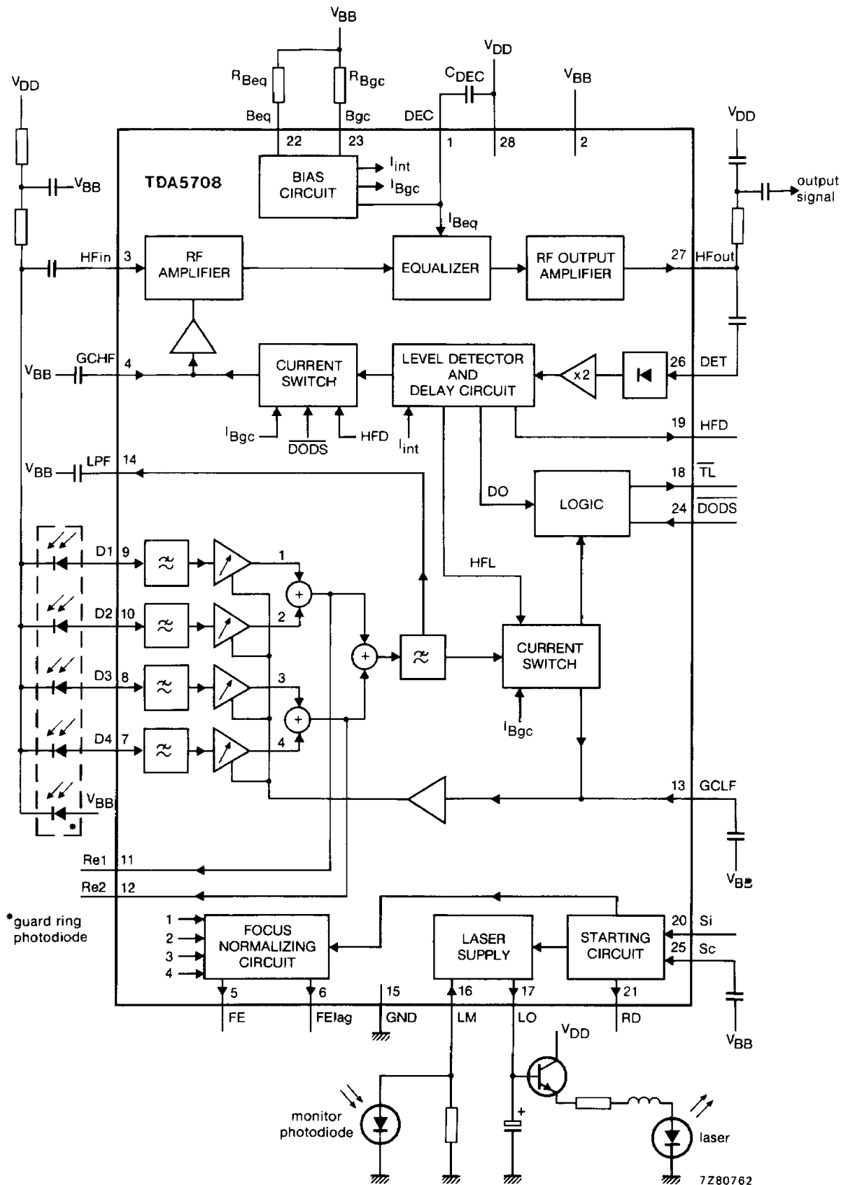
Fig. 1 Block diagram.
