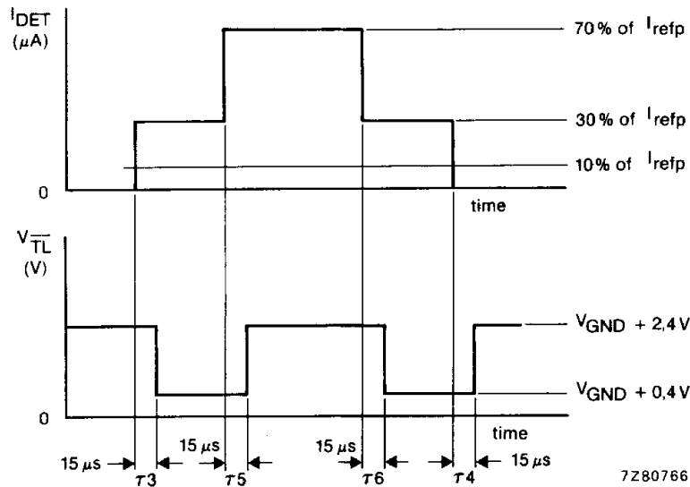
Fig. 5 Delay times between I_{DET} and V_{\overline{TL}} .
