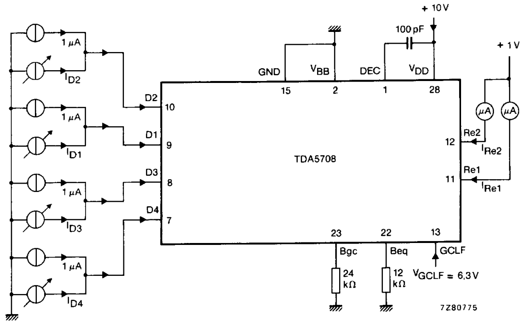
Fig. 14 Test circuit for LF part; a.c. gain.
