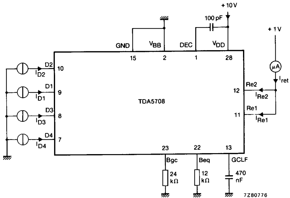
Fig. 15 Test circuit for total reference current I_{ret} .
