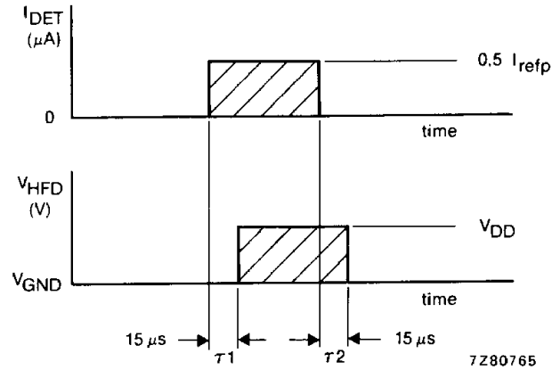
Fig. 4 Delay time \tau between I_{DET} and V_{HFD} .
