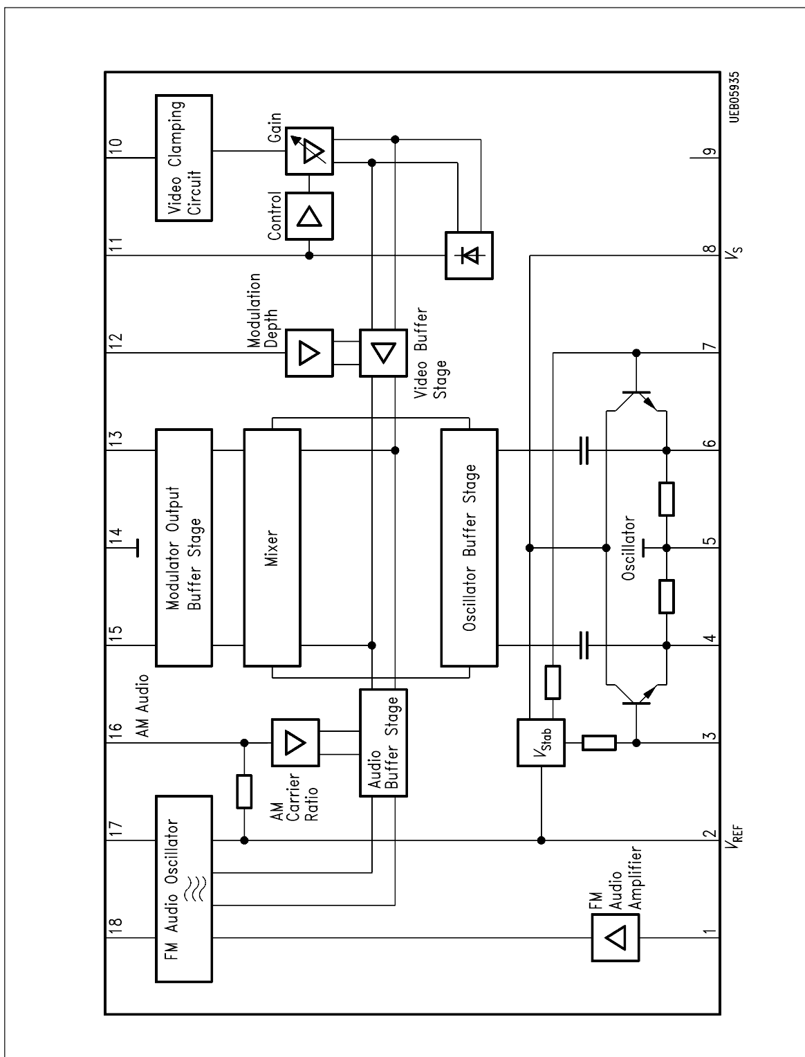
Block Diagram
