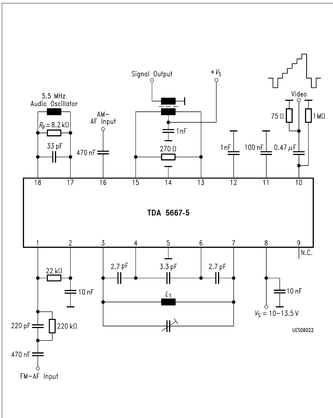
Application Circuit
