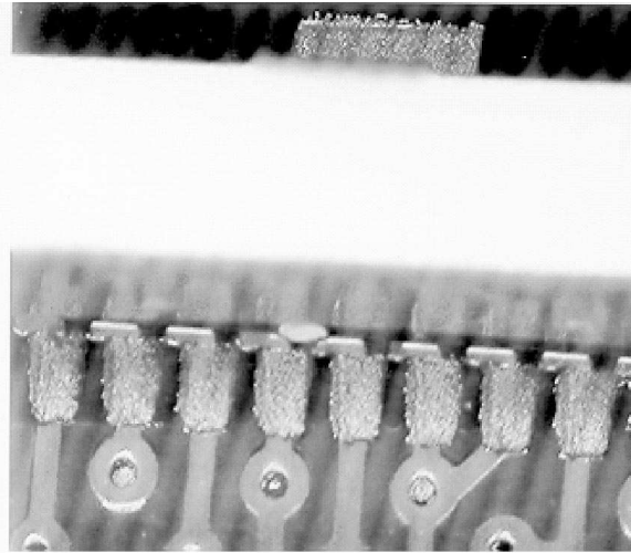
Photo 1.0. Castellations misaligned to land pads in x-axis before reflow.
